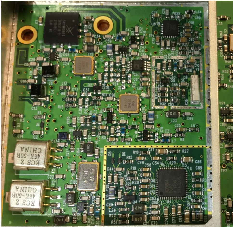
Top view both shields removed
