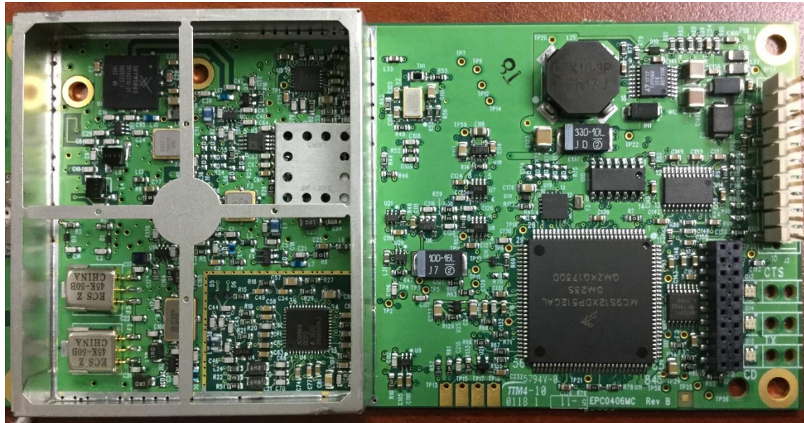
Top view without top shield
