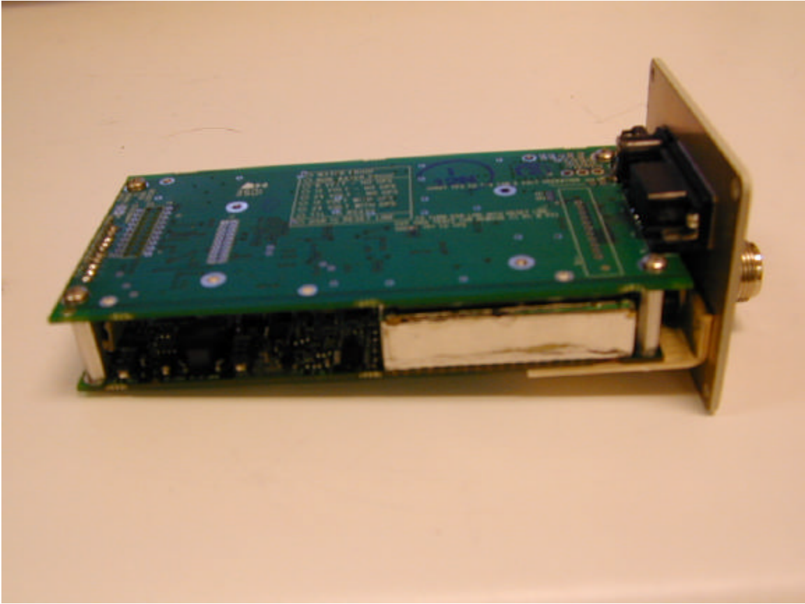
Photo 7. Internal photo, pre-assembled transceiver. Right side view.
