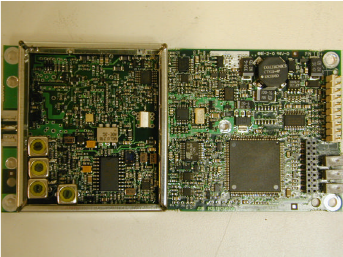
Photo 2. Internal photo. No shield, components labels view.
