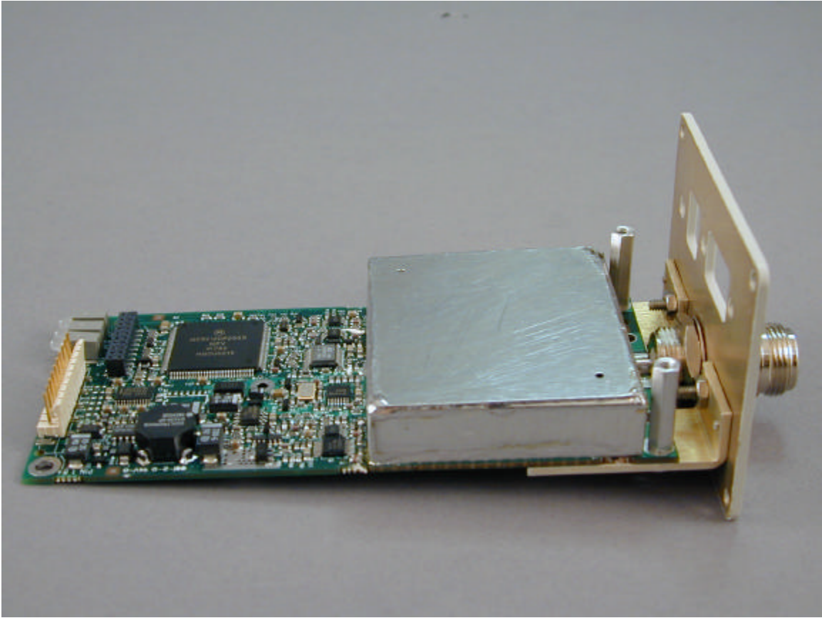
Photo 5. Internal photo. Right side view.
