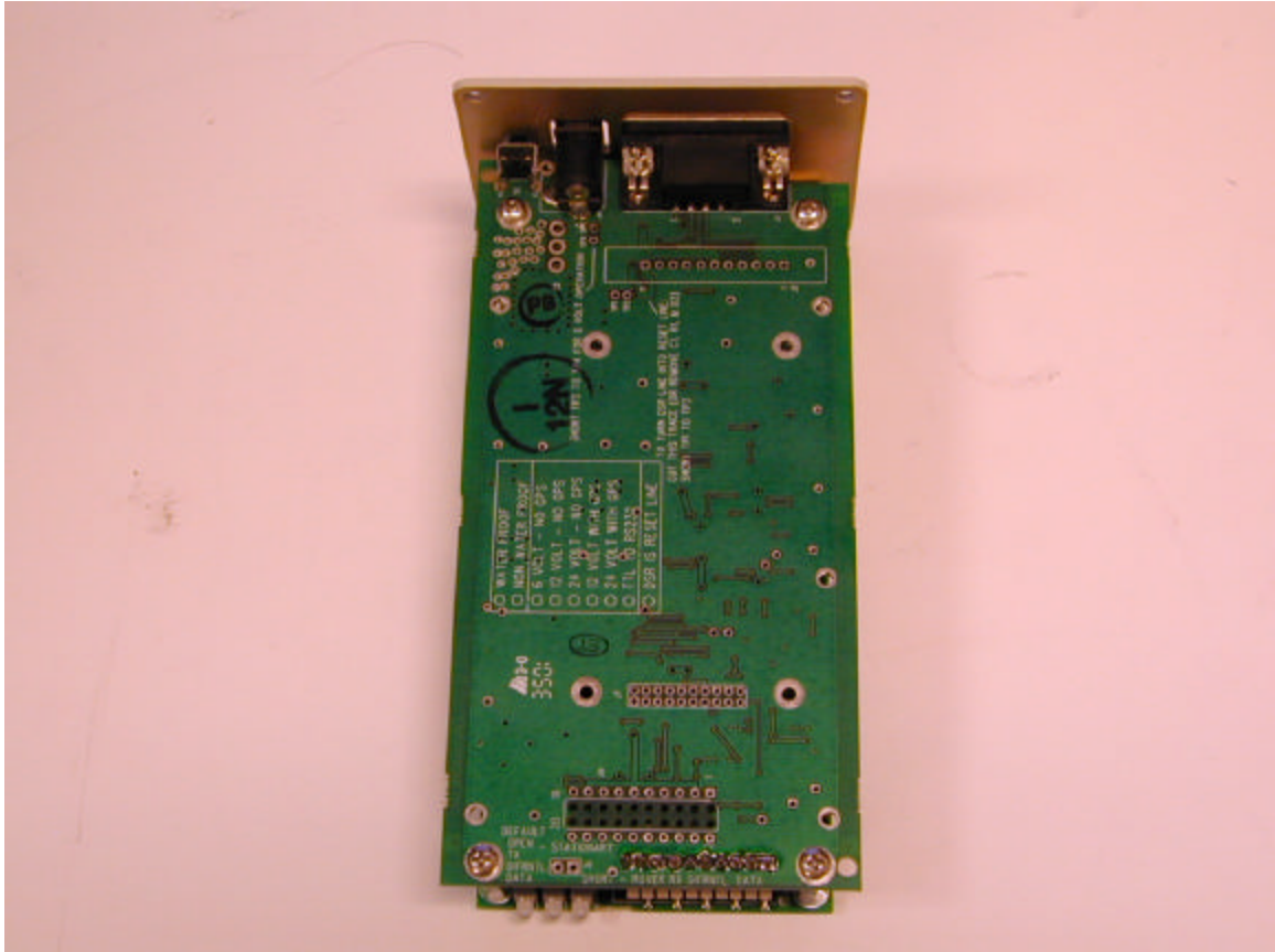
Photo 5. Internal photo, pre-assembled transceiver. Top view.
