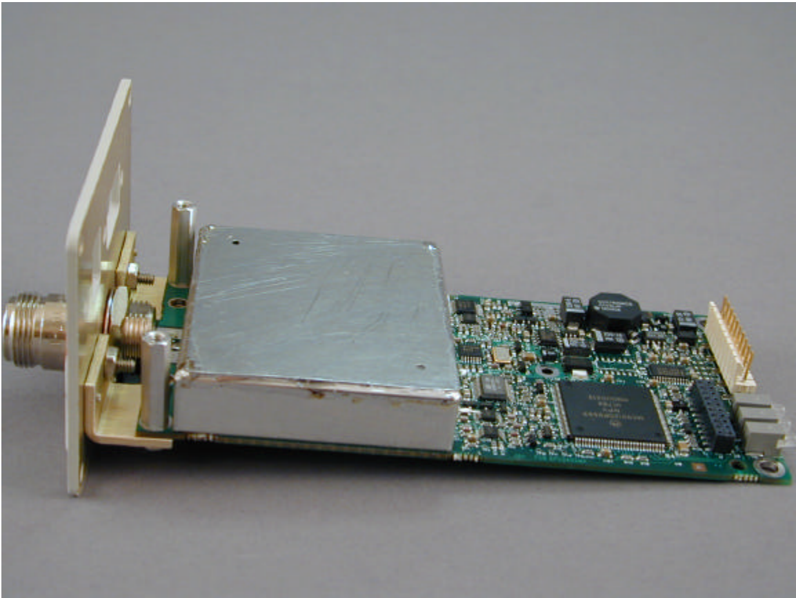
Photo 4. Internal photo. Left side view.
