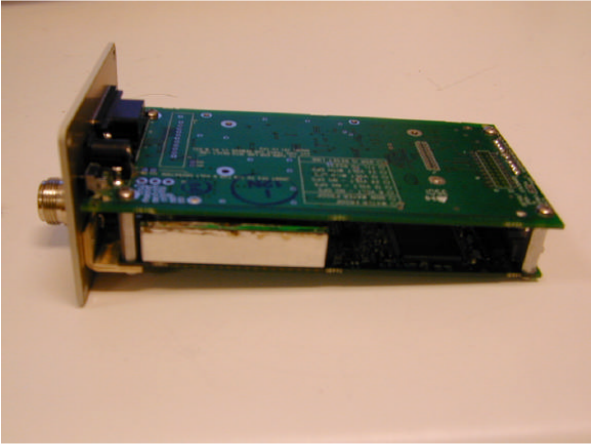
Photo 6. Internal photo, pre-assembled transceiver. Left side view.
