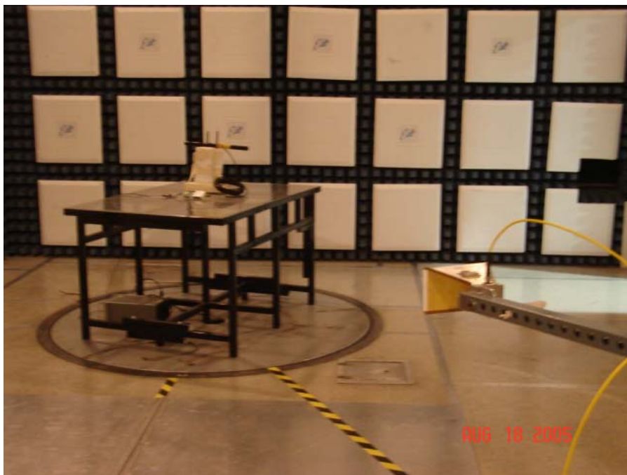
Test Setup for Radiated Emissions with the Yagi Antenna - Vertical Polarization
