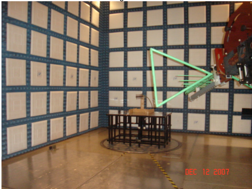
Test Setup for Radiated Emissions Yagi Antenna – Horizontal Polarization
