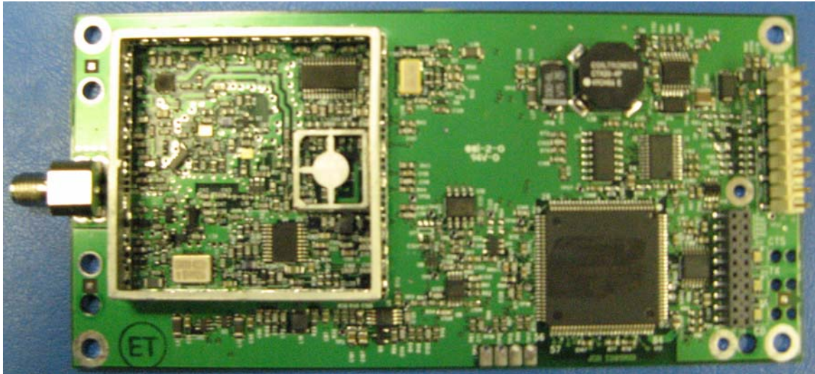
Photo: FGR209 Transceiver Assembly Top w/o Shield
