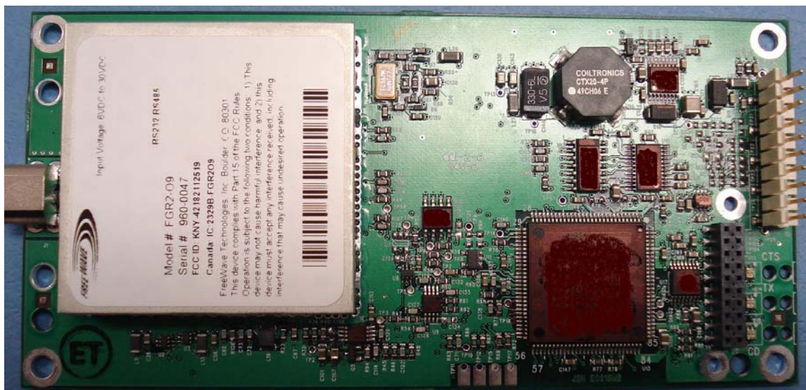
Photo: FGR209 Transceiver Assembly Top w/ shield
