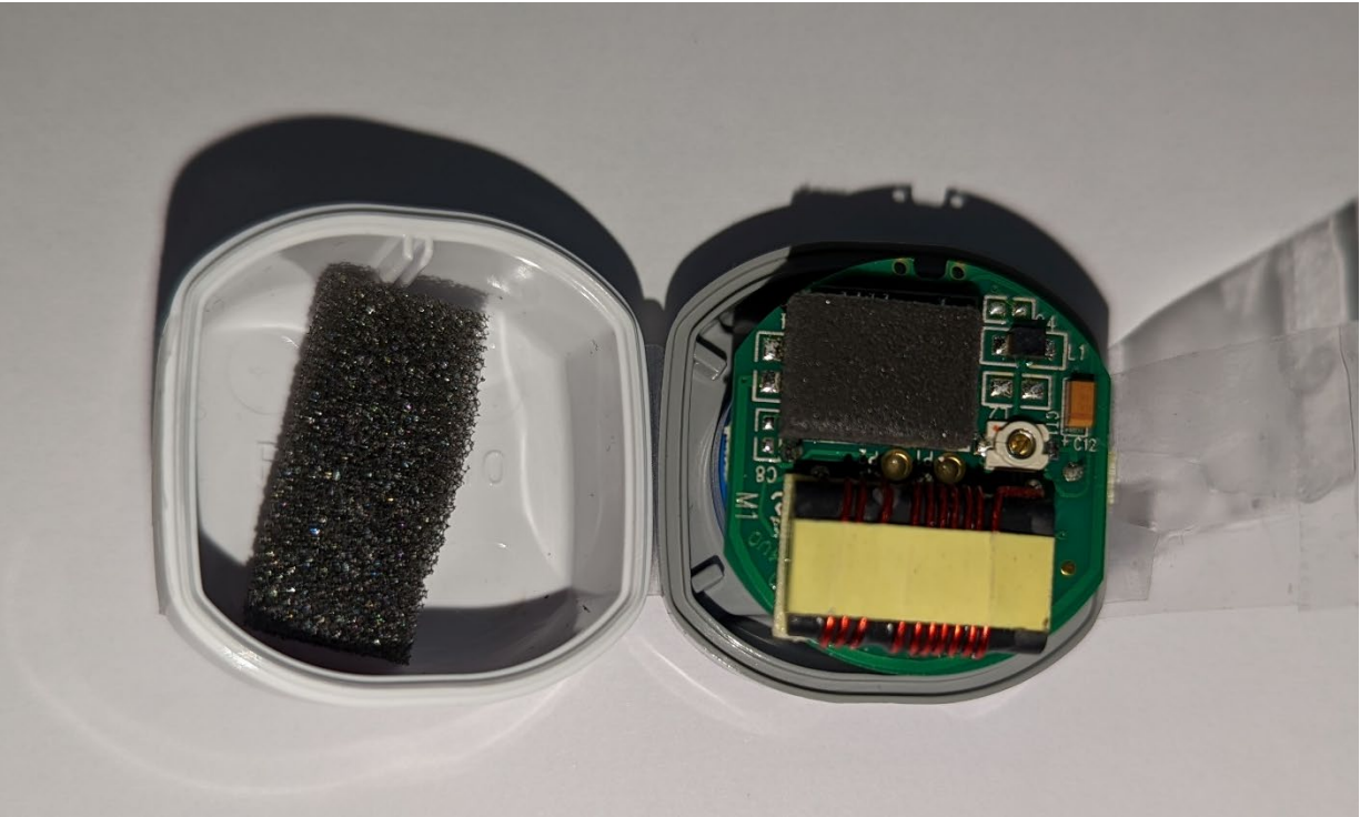
Cover removed
