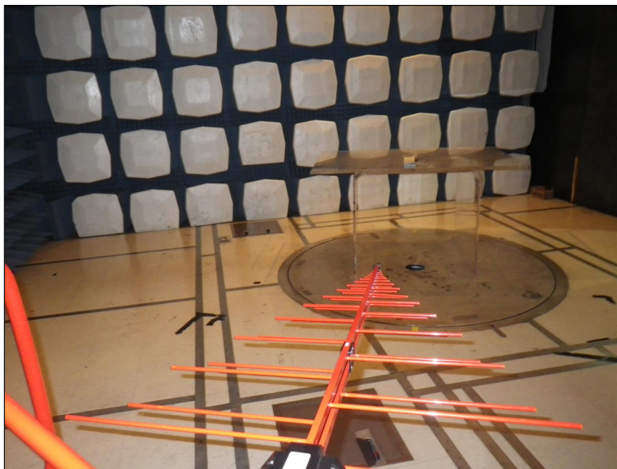
Photograph 4. Radiated Spurious Emissions, Test Setup, 30 MHz – 100 MHz
