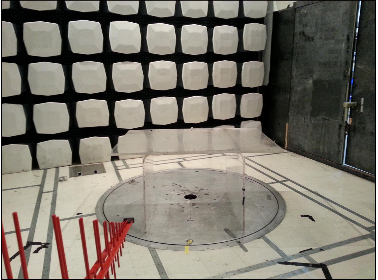
Photograph 1. Radiated Emissions, 30 MHz – 1 GHz, Test Setup
