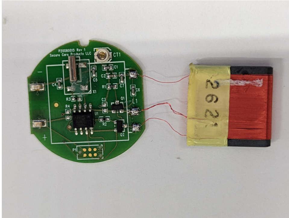
Top Side Antenna Removed
