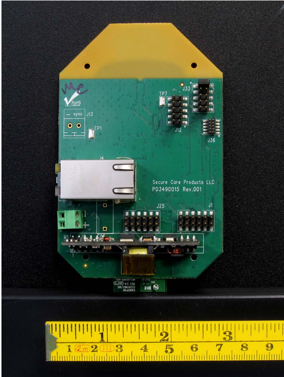
PCB Front
