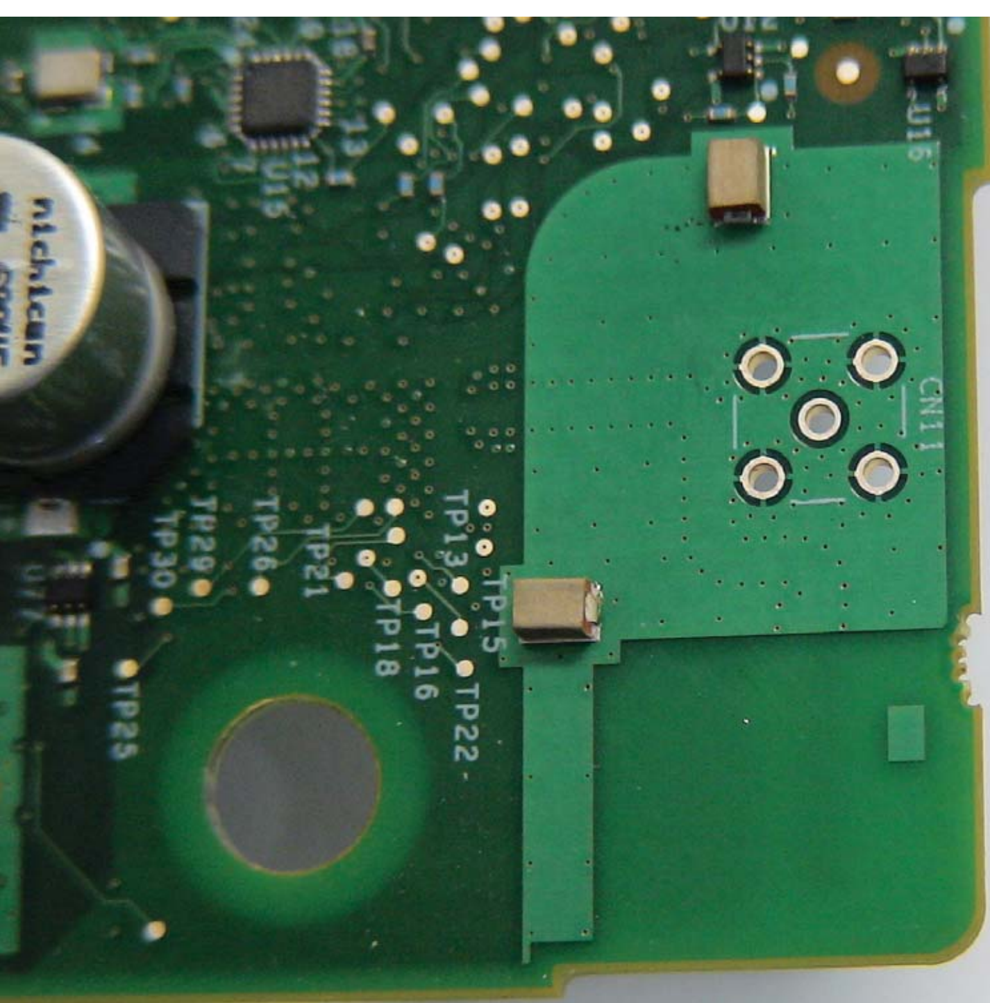
PCB (bottom)
