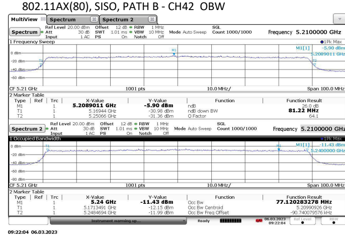
Figure 7: Example Intentional Emission Bandwidth Plots.
