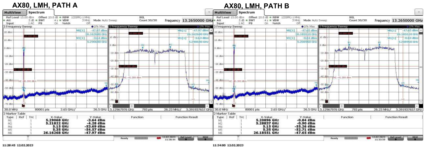
Figure 9(c): Worst Case Transmitter OOB Emissions Measured.
