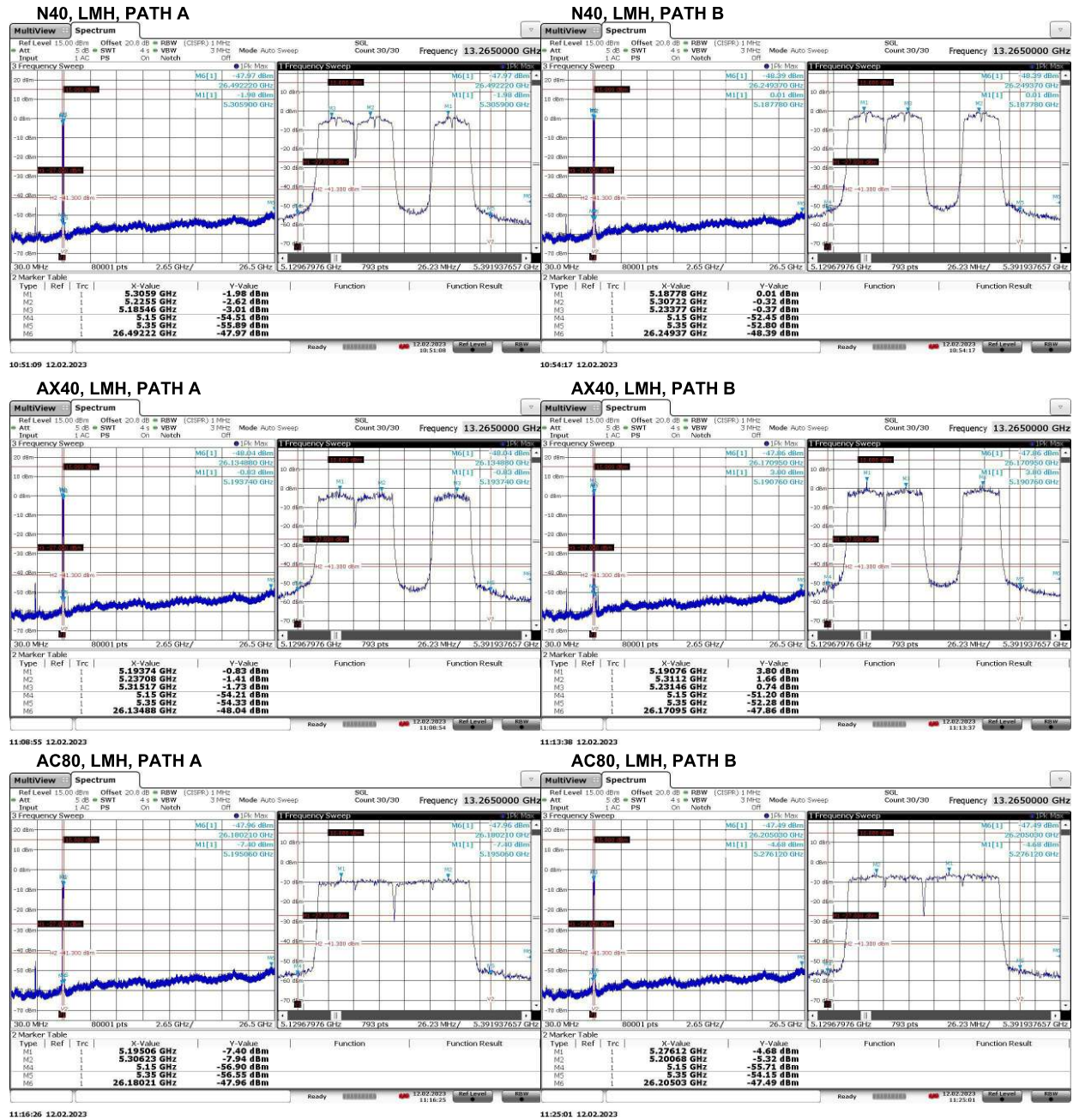
Figure 9(b): Worst Case Transmitter OOB Emissions Measured.
