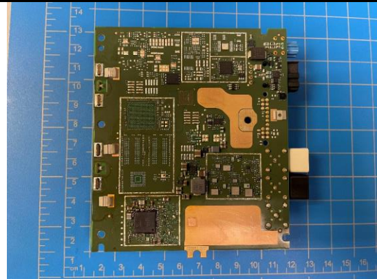
Main board Uncover Bottom View
