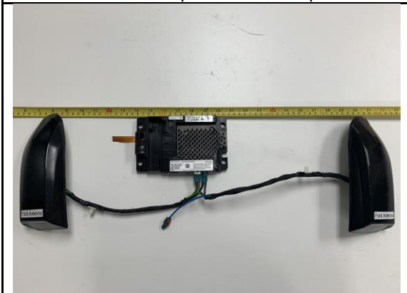
Typical connection (with short RF cable)
