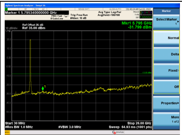
n77_80MHz_Lower Band_Mid Channel
