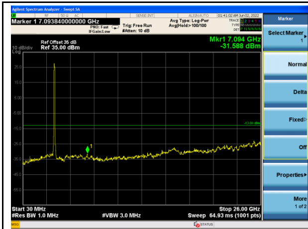
n77_60MHz_Lower Band_Mid Channel
