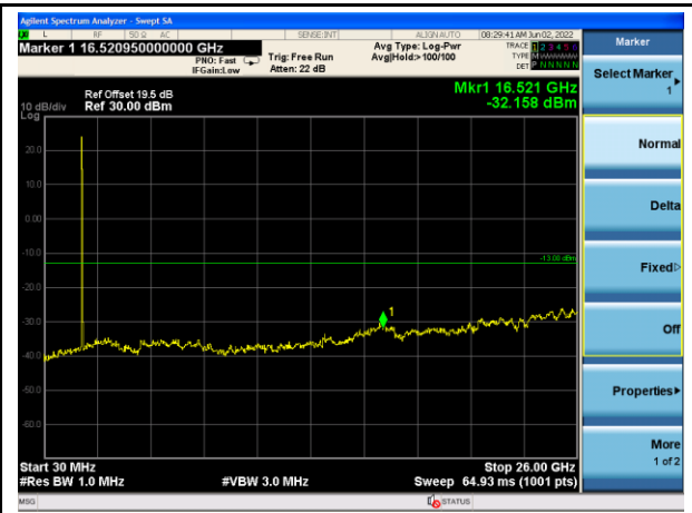
n2_10MHz_Mid Channel
