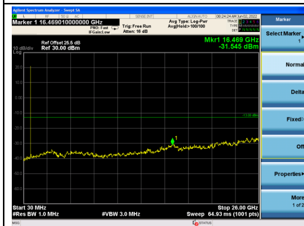
n5_5MHz_Mid Channel
