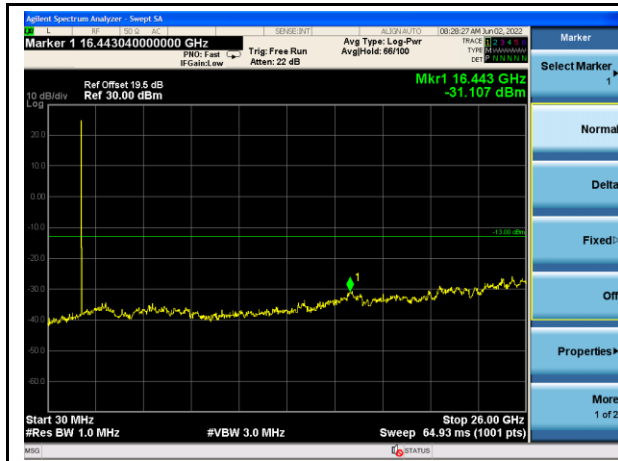
n2_5MHz_Mid Channel
