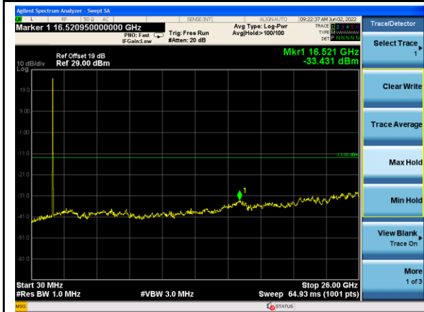
n66_15MHz_Mid Channel
