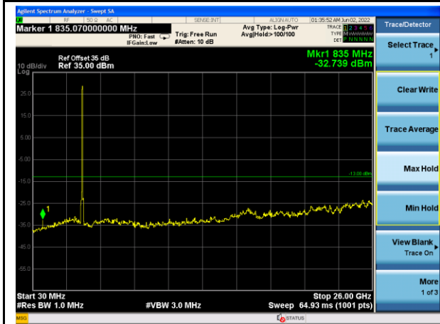
n77_40MHz_Higher Band_Mid Channel
