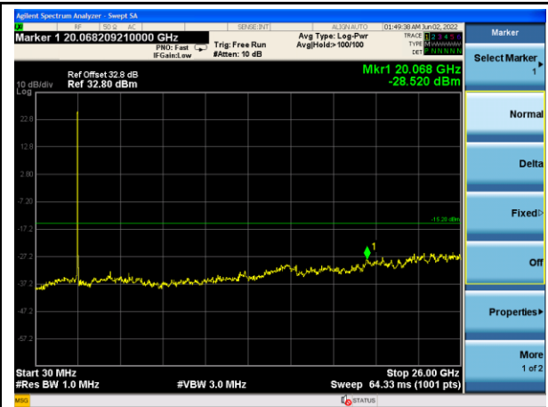
n41_30MHz_Mid Channel
