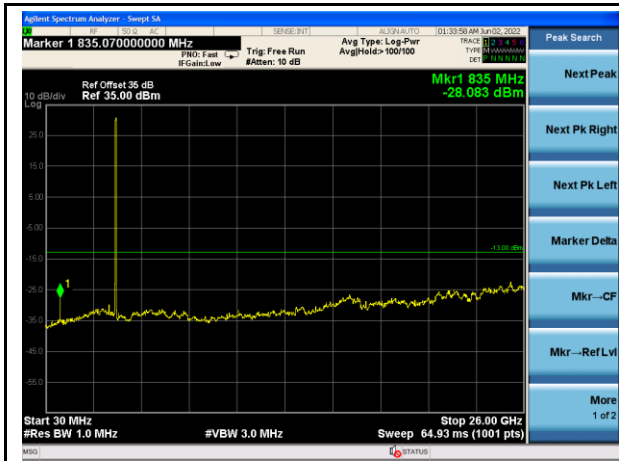
n77_20MHz_Higher Band_Mid Channel
