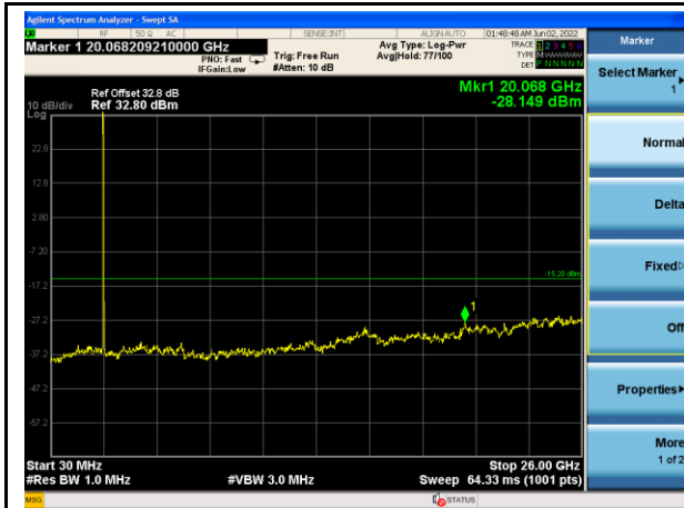
n41_20MHz_Mid Channel
