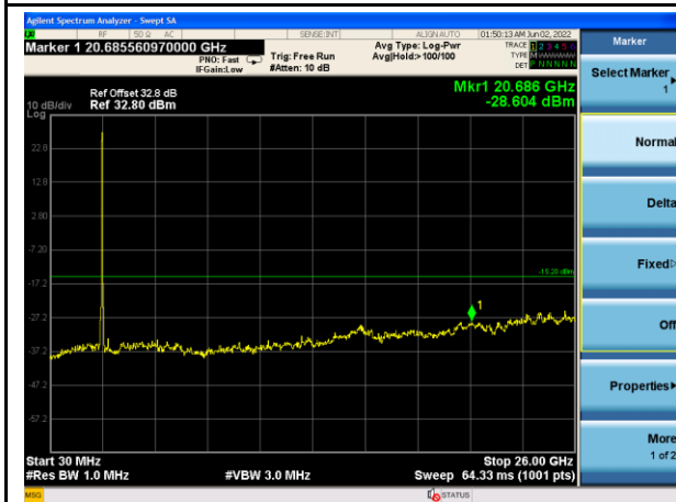
n41_40MHz_Mid Channel
