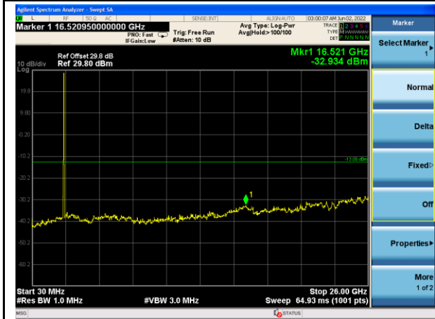
n7_15MHz_Mid Channel
