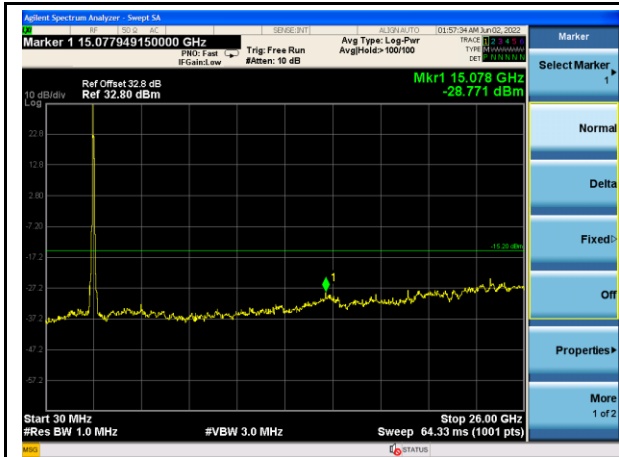
n41_100MHz_Mid Channel
