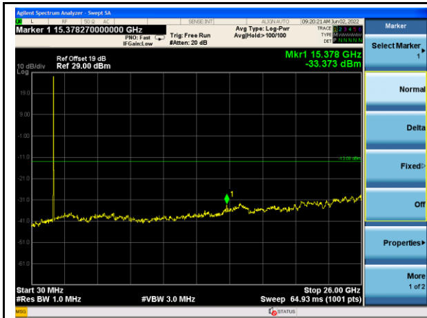
n66_5MHz_Mid Channel
