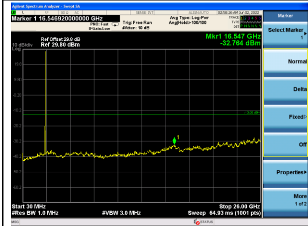
n7_5MHz_Mid Channel
