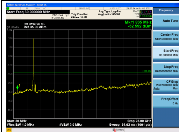
n77_80MHz_Higher Band_Mid Channel
