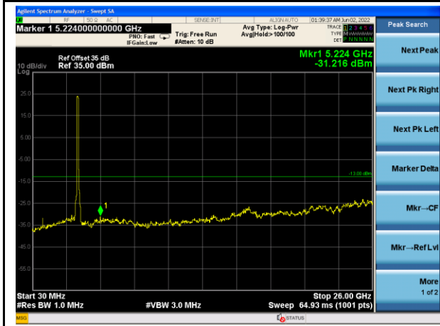
n77_100MHz_Lower Band_Mid Channel
