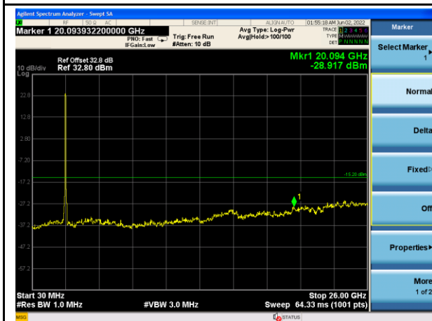
n41_60MHz_Mid Channel
