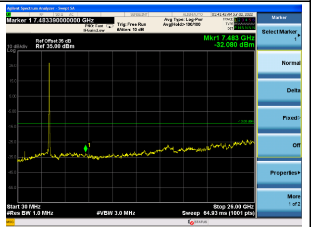
n77_50MHz_Lower Band_Mid Channel
