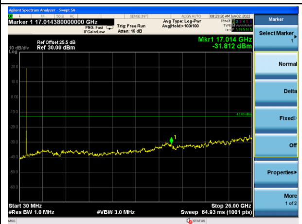
n5_10MHz_Mid Channel
