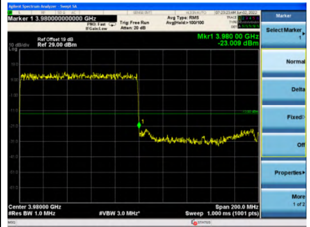
n77_Higher Band_100MHz_Upper Band Edge
