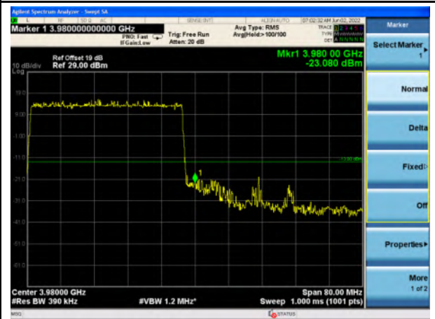
n77_Higher Band_40MHz_Upper Band Edge
