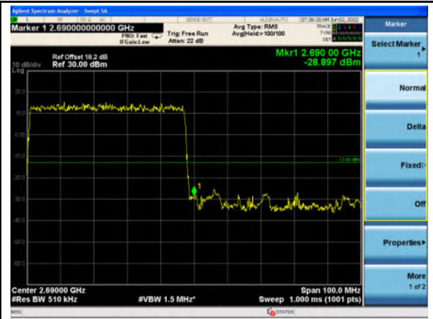
n41_50MHz_Upper Band Edge
