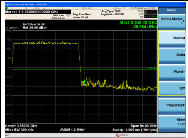
n77_Low Band_40MHz_Upper Band Edge
