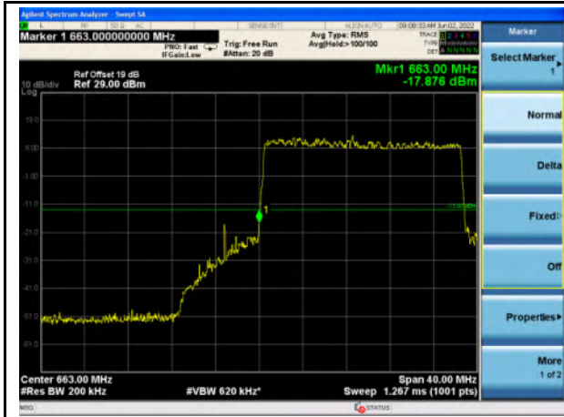
n71_20MHz_Lower Band Edge
