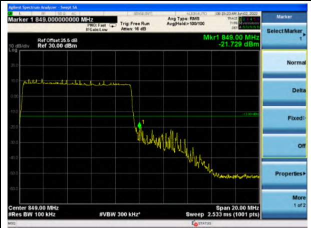
n5_10MHz_Upper Band Edge
