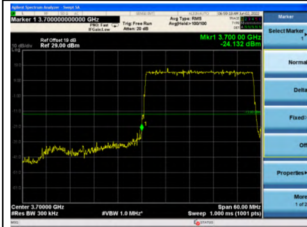
n77_Higher Band_30MHz_Lower Band Edge
