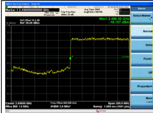
n41_100MHz_Lower Band Edge
