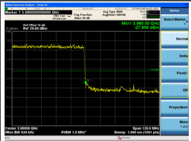
n77_Higher Band_60MHz_Upper Band Edge
