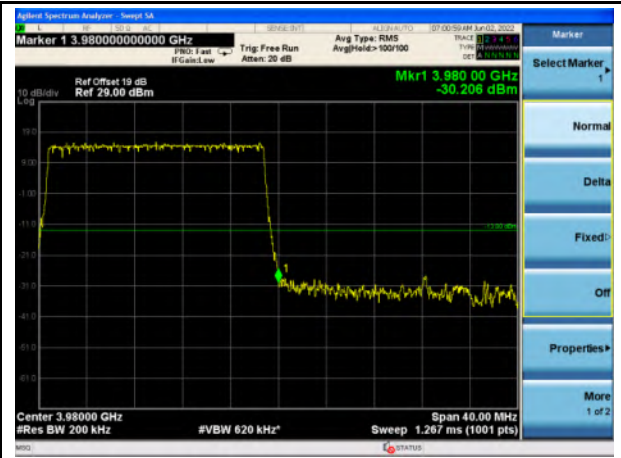
n77_Higher Band_20MHz_Upper Band Edge
