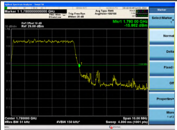
n66_5MHz_Upper Band Edge
