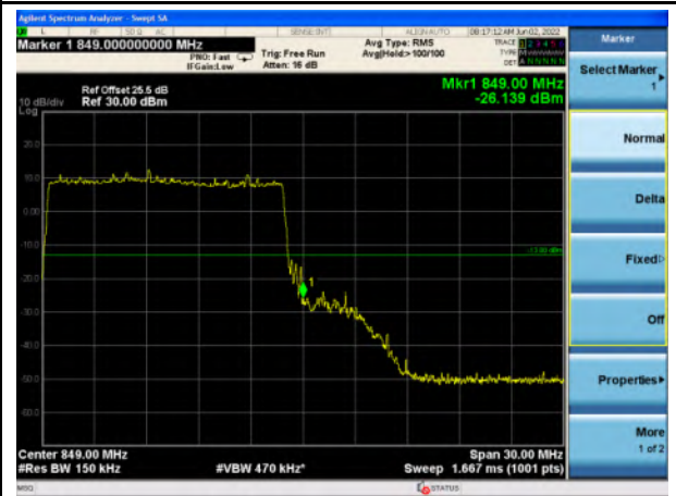
n5_15MHz_Upper Band Edge
