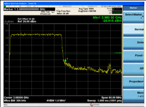
n77_Higher Band_30MHz_Upper Band Edge
