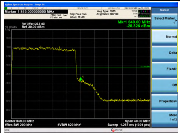
n5_20MHz_Upper Band Edge
