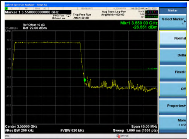
n77_Low Band_20MHz_Upper Band Edge
