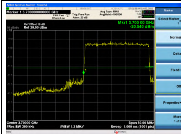
n77_Higher Band_40MHz_Lower Band Edge
