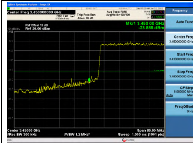
n77_Low Band_40MHz_Lower Band Edge
