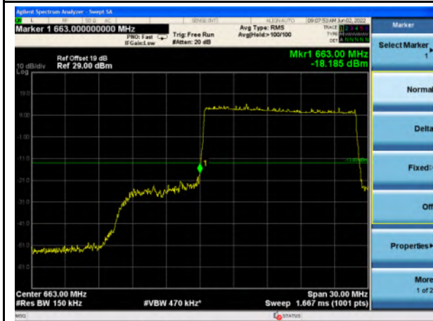
n71_15MHz_Lower Band Edge
