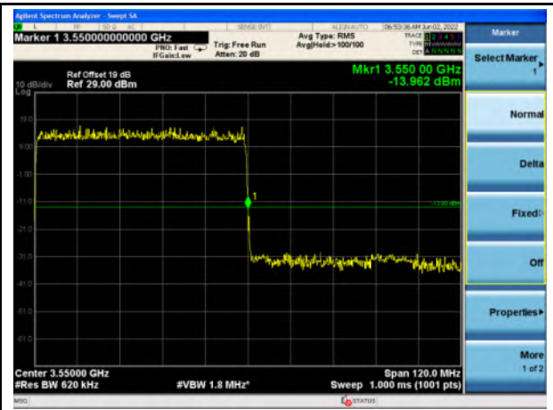
n77_Low Band_60MHz_Upper Band Edge
