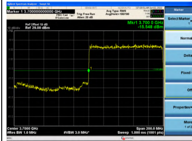
n77_Higher Band_100MHz_Lower Band Edge
