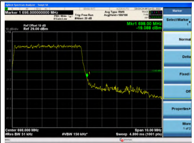
n71_5MHz_Upper Band Edge
