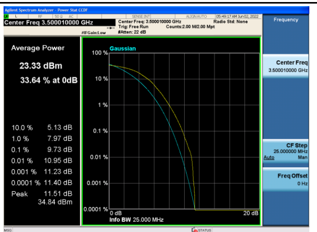
64QAM_20MHz_Mid_Full RB
