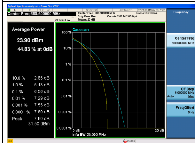
256QAM_20MHz_Mid_Full RB
