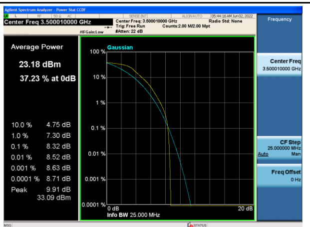
QPSK_20MHz_Mid_Full RB
