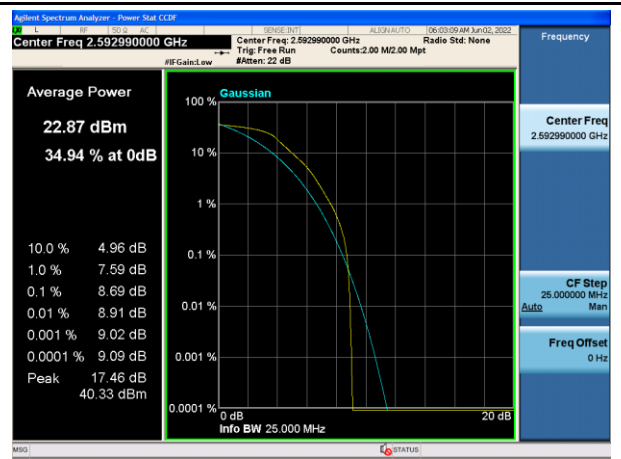
QPSK_20MHz_Mid_Full RB
