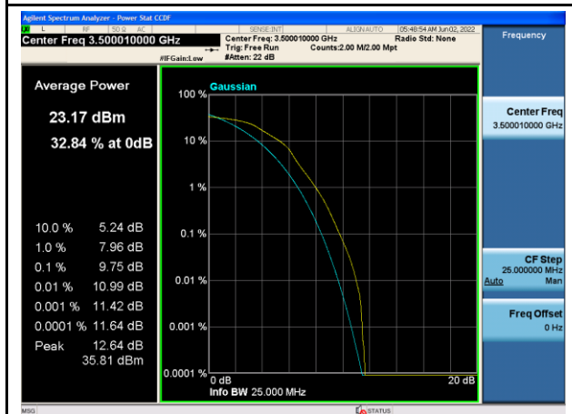
16QAM_20MHz_Mid_Full RB
