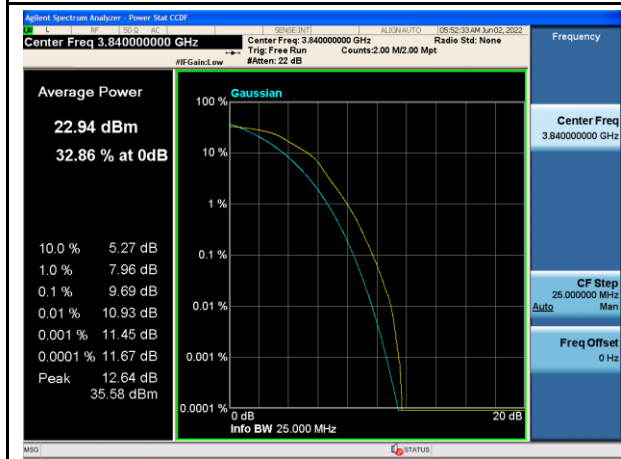
16QAM_20MHz_Mid_Full RB
