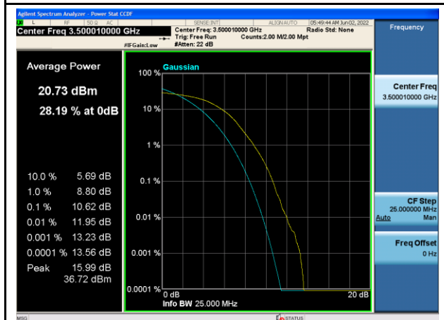
256QAM_20MHz_Mid_Full RB
