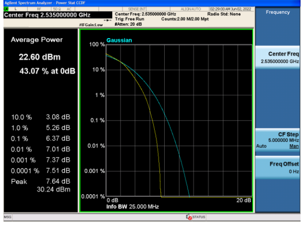
64QAM_20MHz_Mid_Full RB
