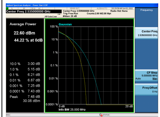
16QAM_20MHz_Mid_Full RB
