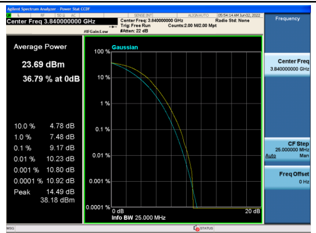
64QAM_20MHz_Mid_Full RB
