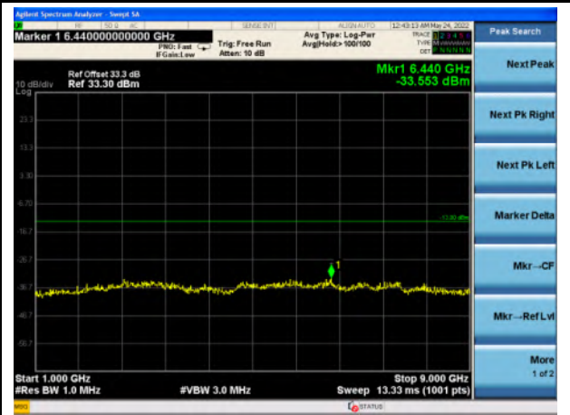
Band 5_QPSK_10M - Mid- 1GHz~9GHz
