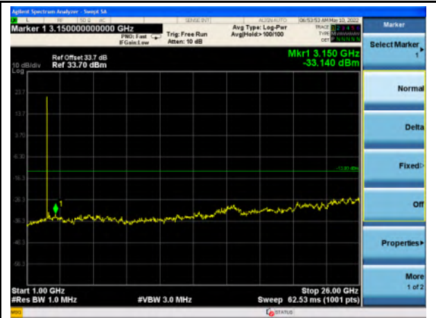
Band 7_QPSK_5M - Mid- 1GHz~26GHz
