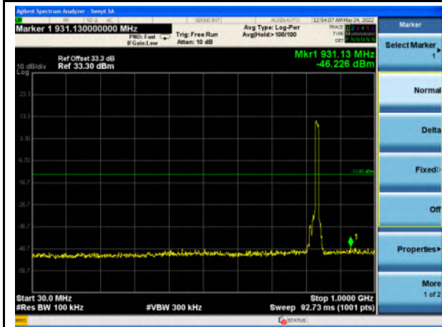
Band 5_QPSK_10M_Mid - 30MHz~1GHz
