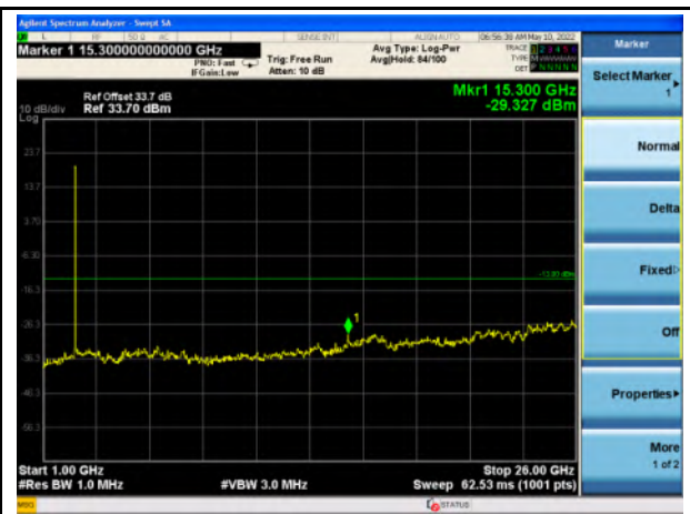
Band 7_QPSK_10M - Mid- 1GHz~26GHz
