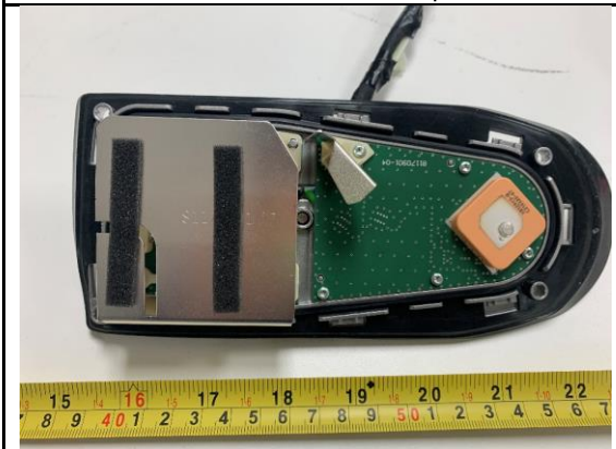
External rooftop antenna#1 - Top View
