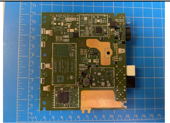
Main board Uncover Bottom View
