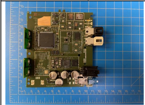
Main board Uncover Top View
