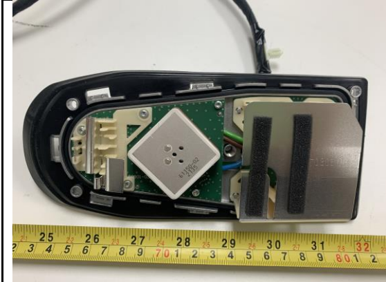
External rooftop antenna#2 - Top View
