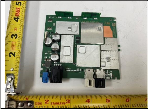
Main board Top View
