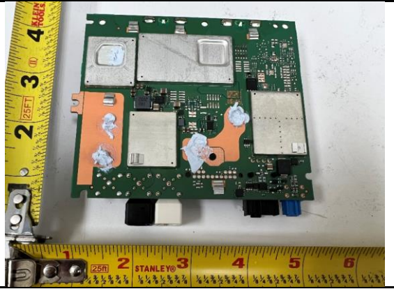
Main board Bottom View
