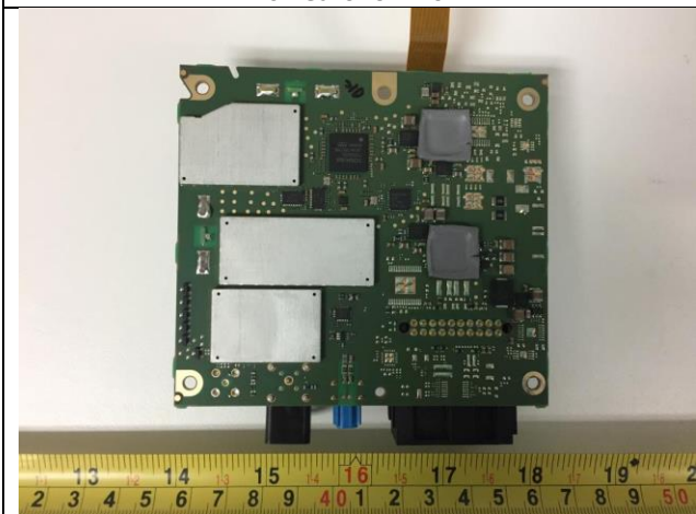
Main PCBA Bottom
