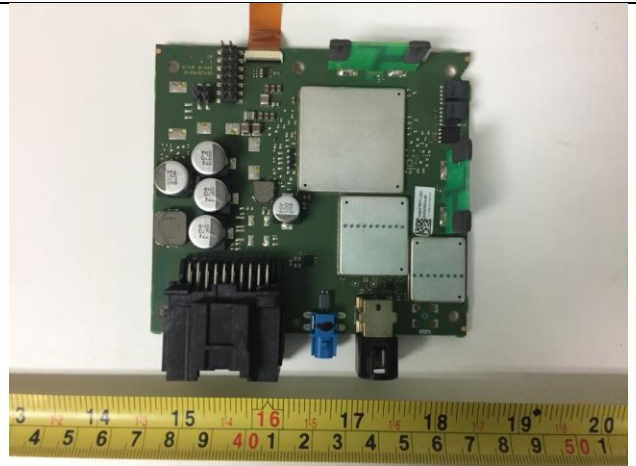
Main PCBA Top
