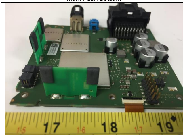
Main PCBA - Internal Antenna 1 (RF Path 0)
