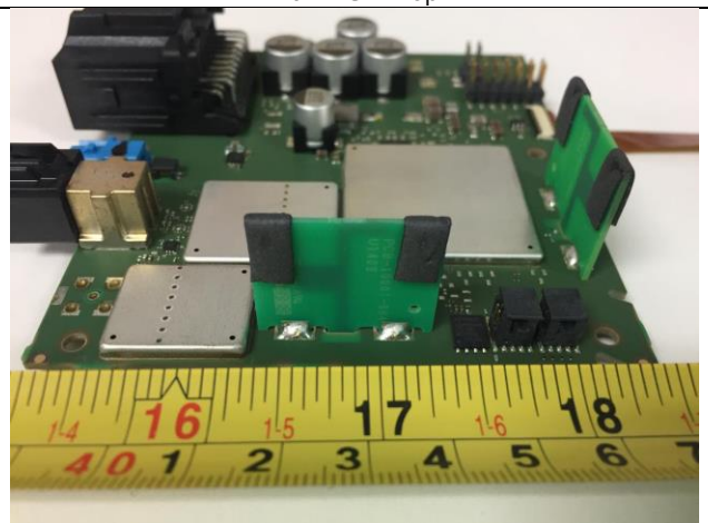
Main PCBA - Internal Antenna 2 (RF Path 1)
