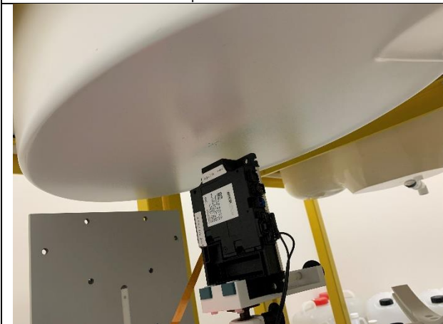
Test Setup - Side (Ant2) Position
