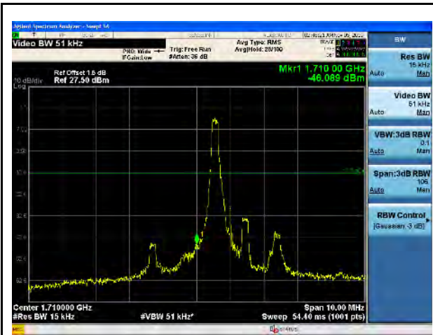
LTE Band 4, 16QAM, 1.4MHz-Low CH, 1RB
