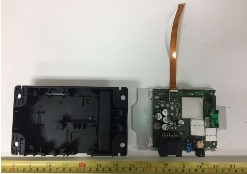
EUT Cover Off View
