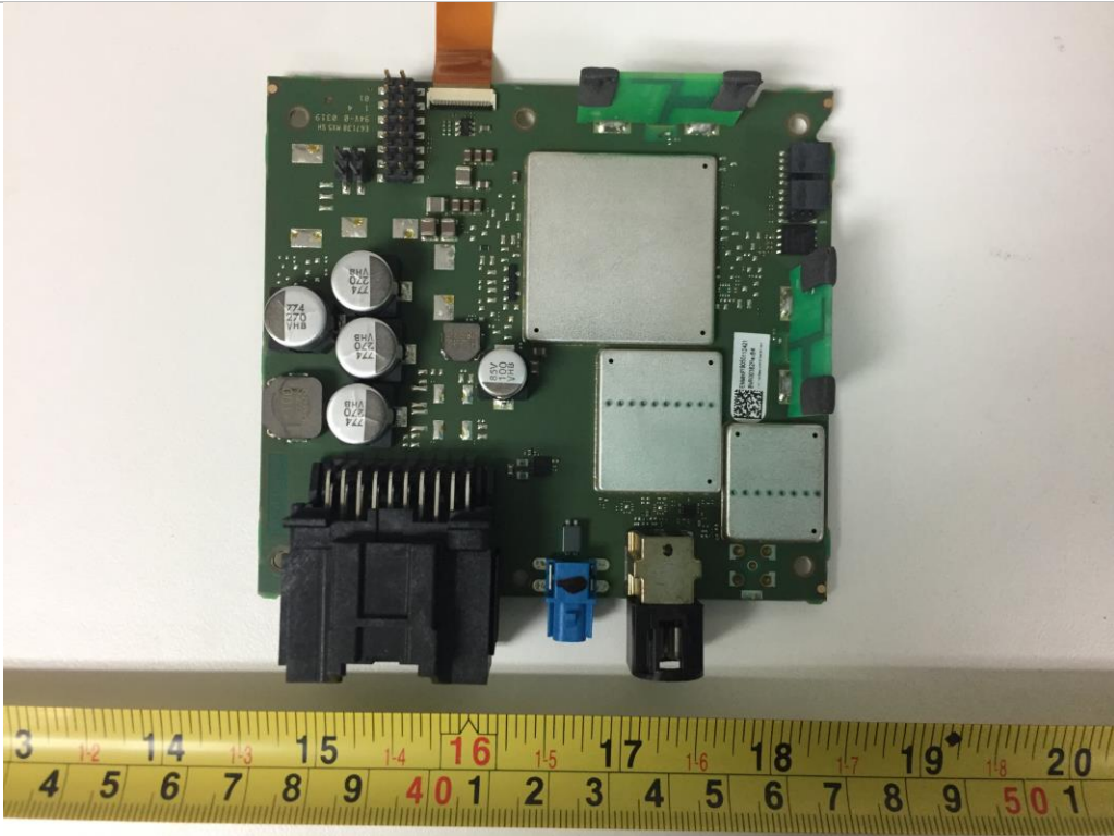
Main PCBA-Top
