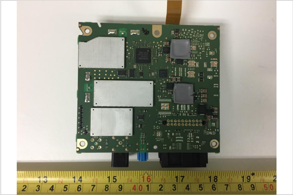
Main PCBA-Bottom
