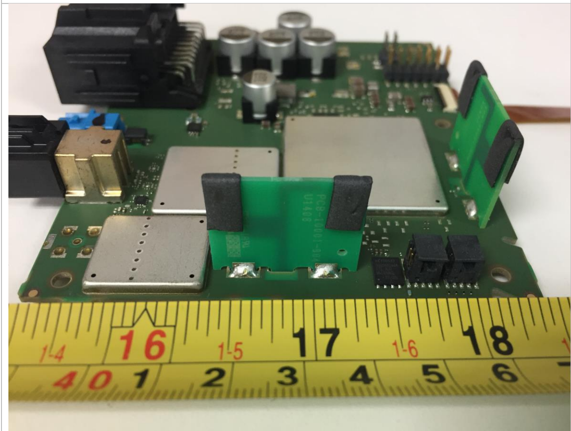
Main PCBA-Internal antenna-1
