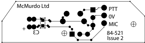
SOLDER SIDE
