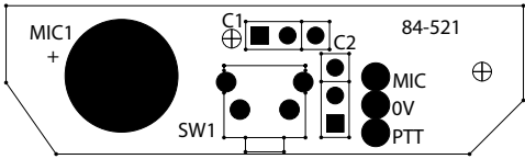
COMPONENT SIDE
