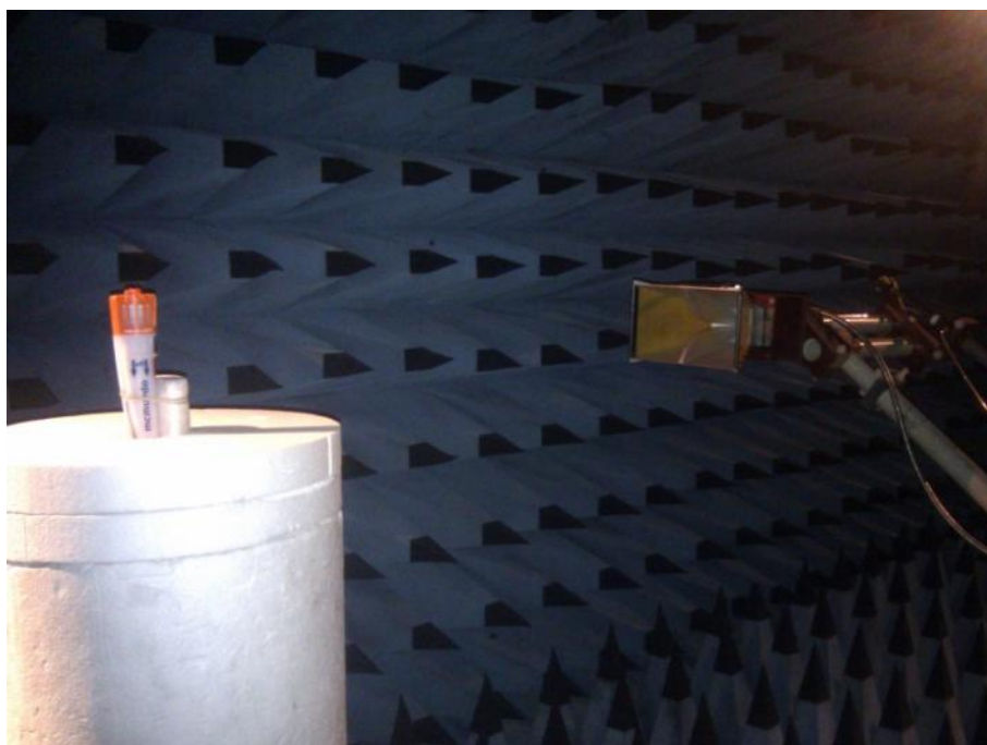
Test Set-up – Z502
