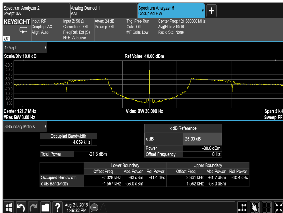
Figure 14 - 99% Occupied Bandwidth
