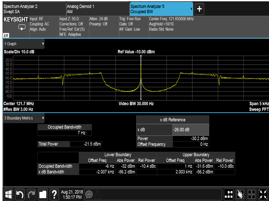
Figure 15 - 30% Occupied Bandwidth
