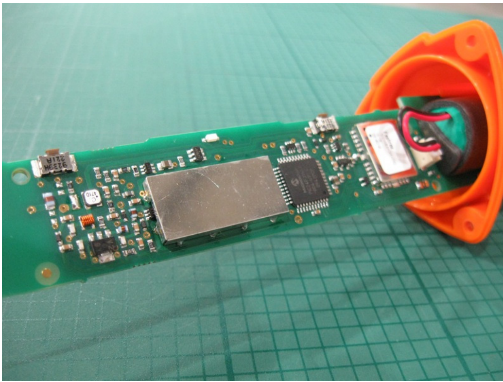
McMurdo Smartfind S5 - PCB components and battery
