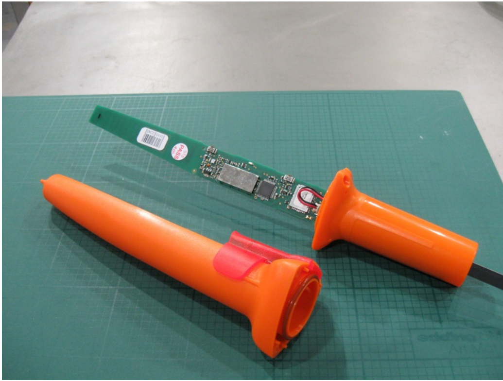
McMurdo Smartfind S5 - component side view
