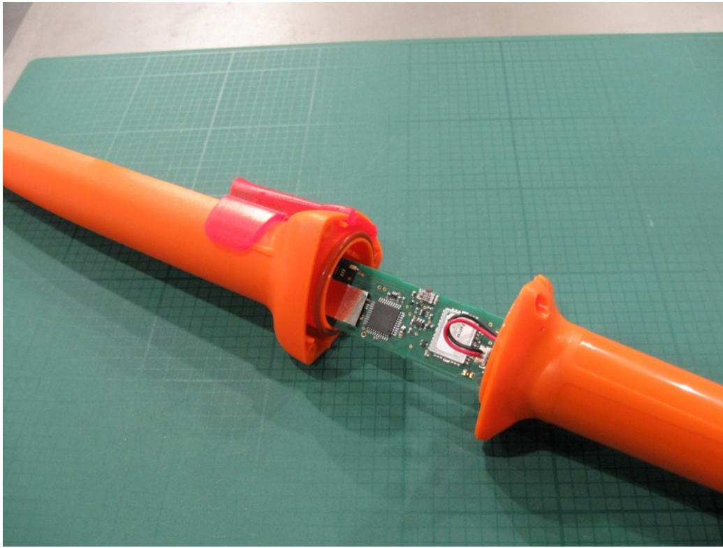
McMurdo Smartfind S5 AIS-SART
