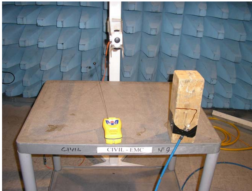
Radiated Immunity Test Setup Orientation 1
