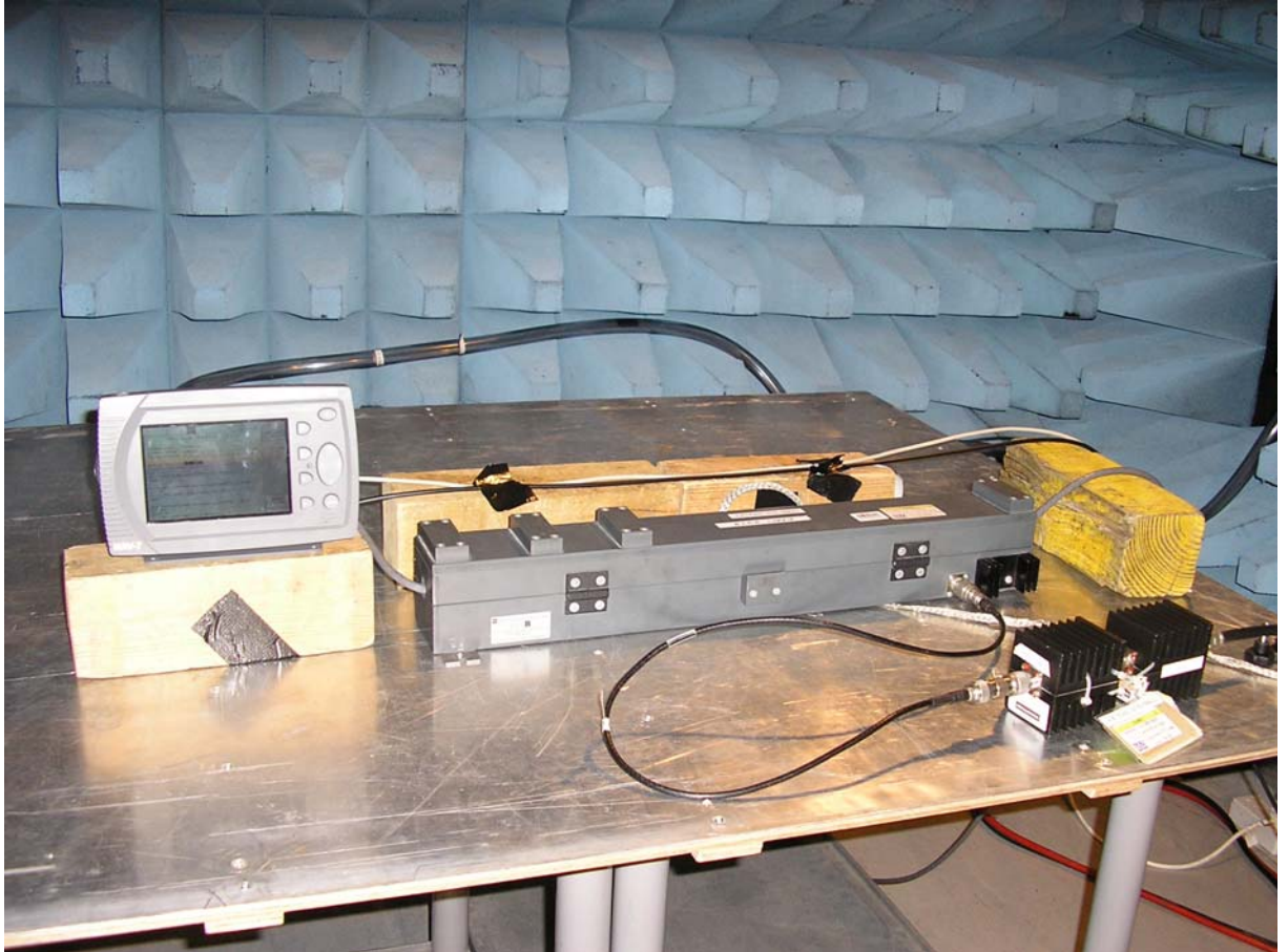
Conducted Immunity Setup
