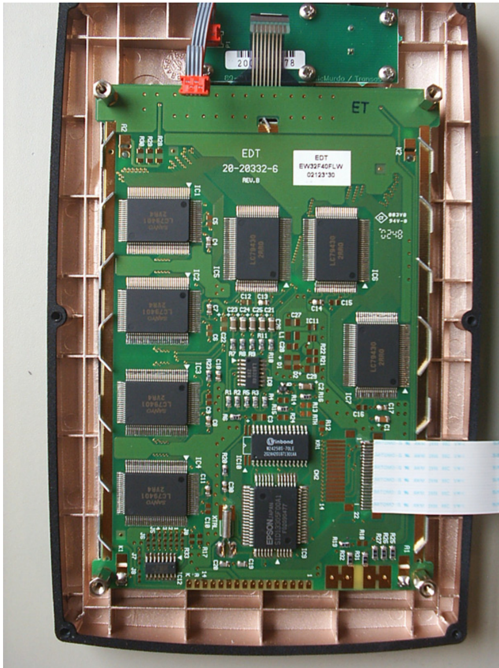
Photograph 14: Display LCD module PCB
