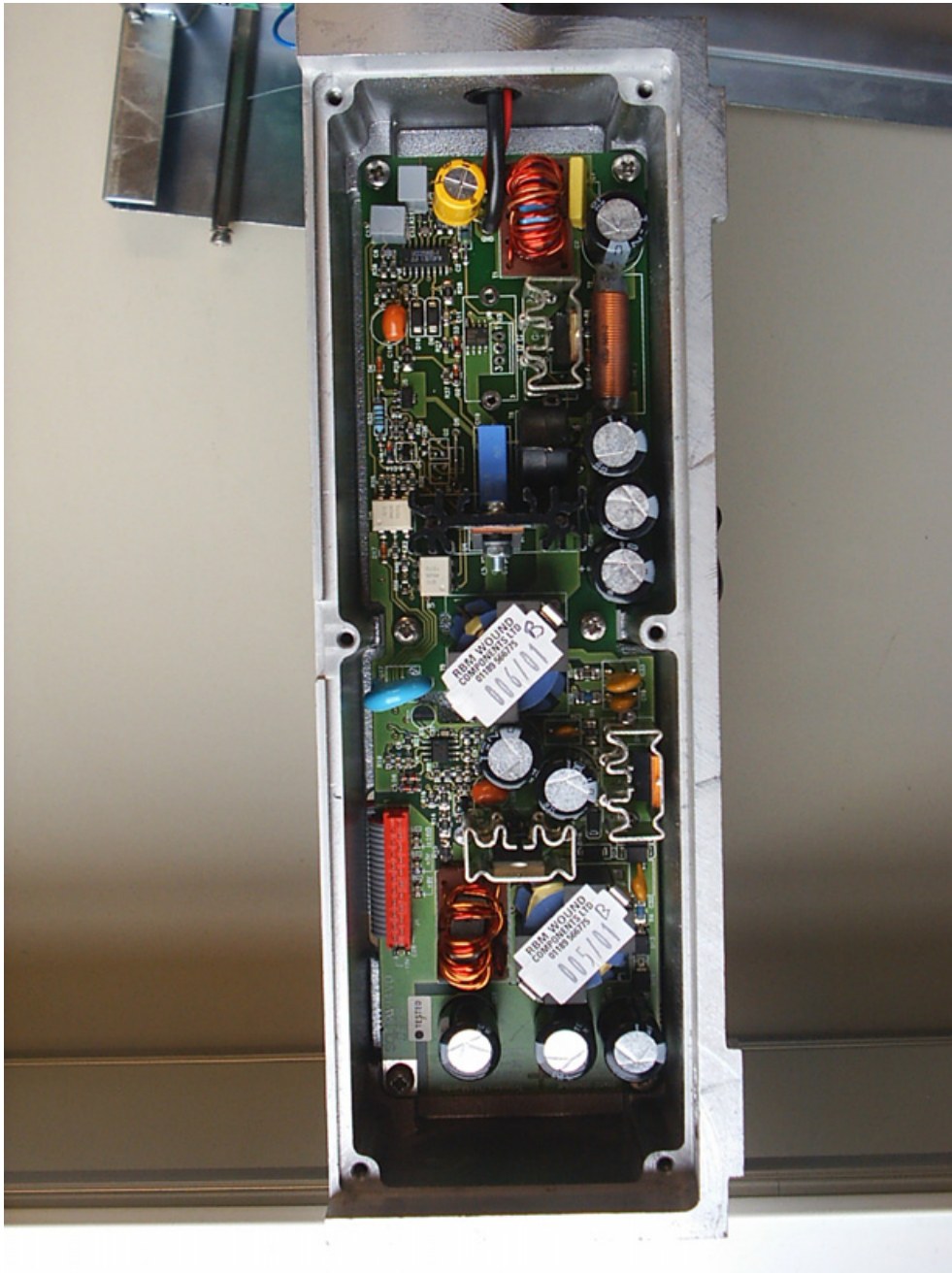
Photograph 11: Power supply
