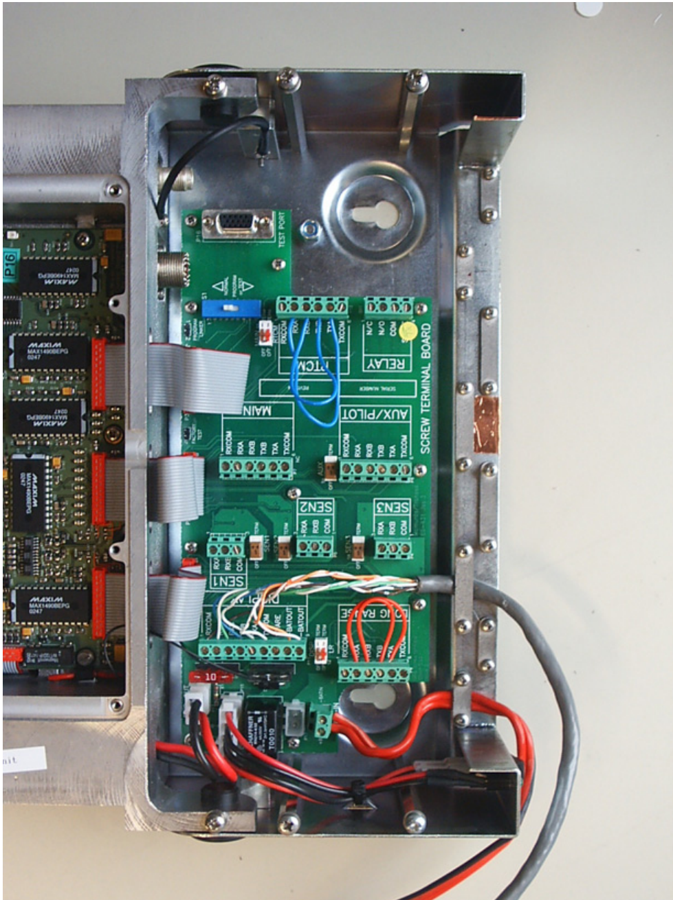
Photograph 12: Screw terminal board
