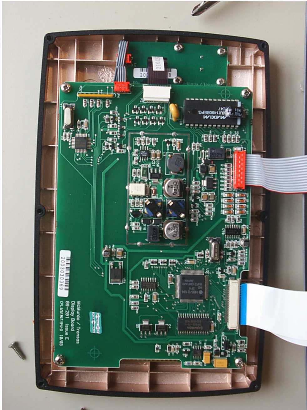
Photograph 13: Display main PCB
