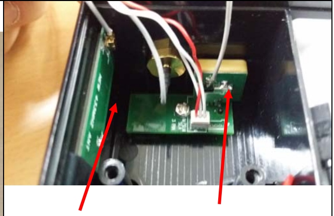
433 Antenna
