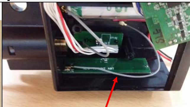
433 MHz Antenna
