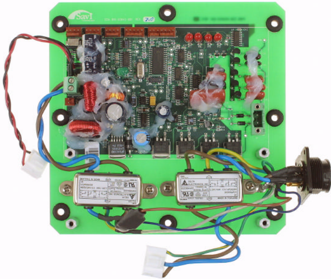
Main Circuit Board – Bottom and Top
