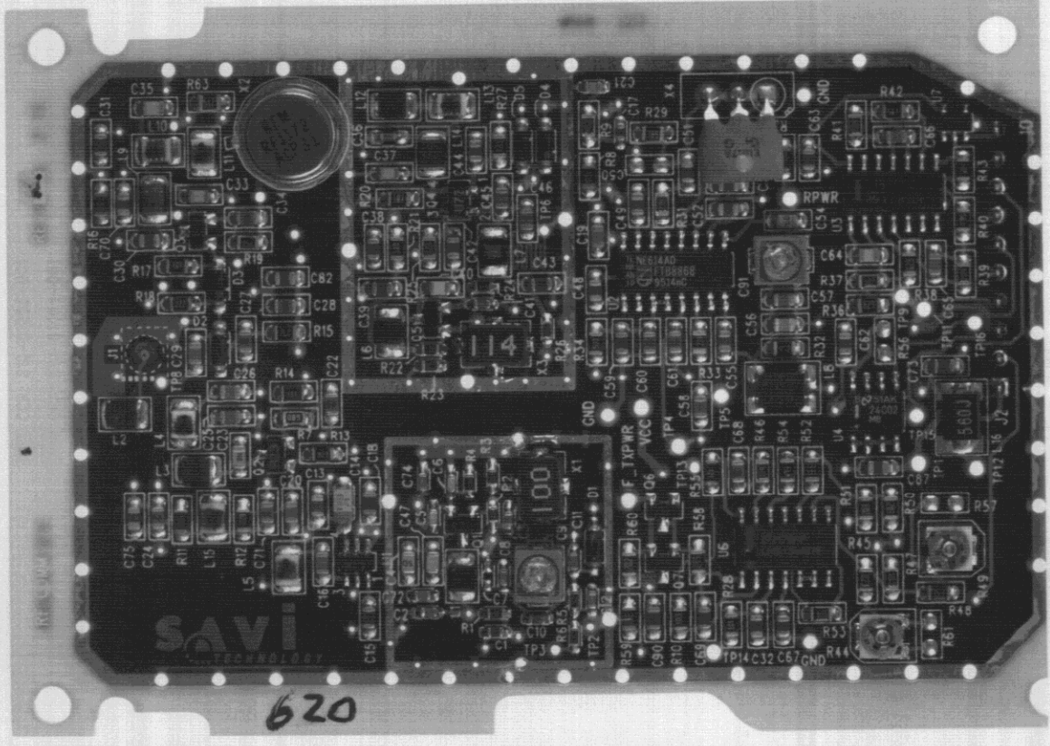
Savi Technology FCC ID: KL7-410GR-V11 RF Communications Board Top w/ and w/o Shield
