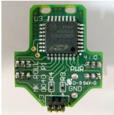
Daughter Board Top
