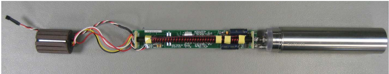
Board with Sensor Module and Battery Housing
