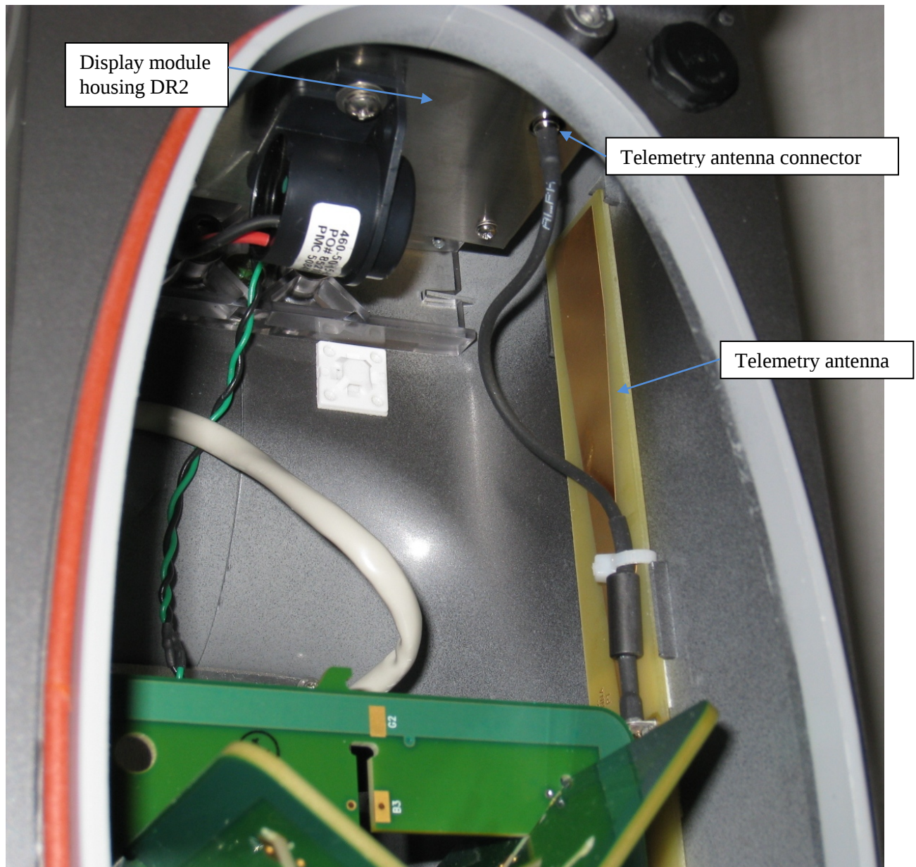
Front cover off showing placement of telemetry antenna and connection to DR2
