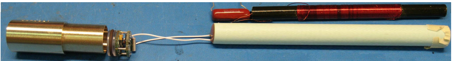
PCB assembly with antenna assembly (antenna and capacitor shown above are what is inside the long potted tube)
