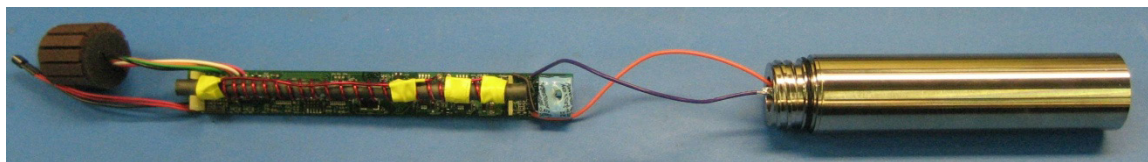
Board with Roll/Pitch Sensor Module and Battery Housing
