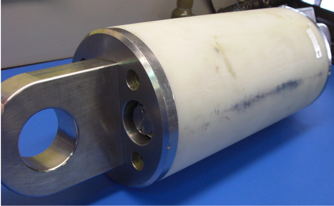
TT Side 2 and Front end, top, showing pressure sensor
