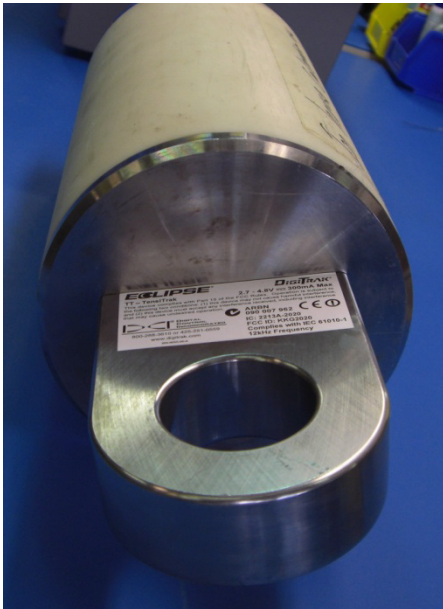
TensiTrak Rear End, top, Showing Eclipse Label
