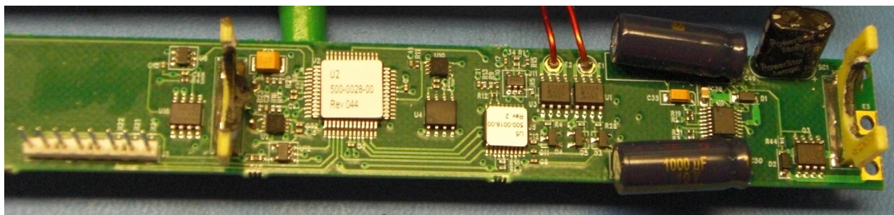
Right Top 2, antenna removed
