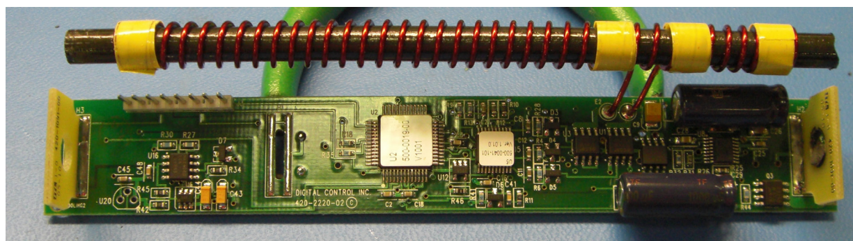
Circuit board top, antenna removed
