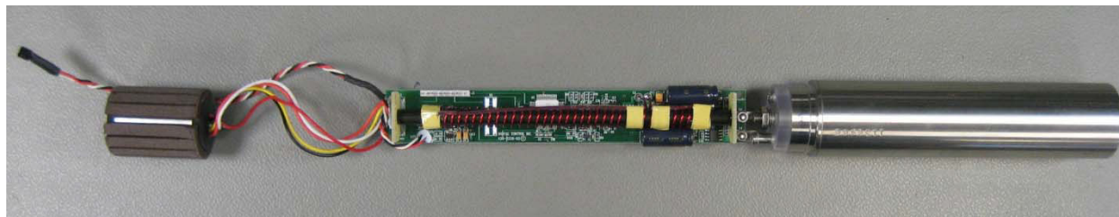
Board with Sensor Module and Battery Housing
