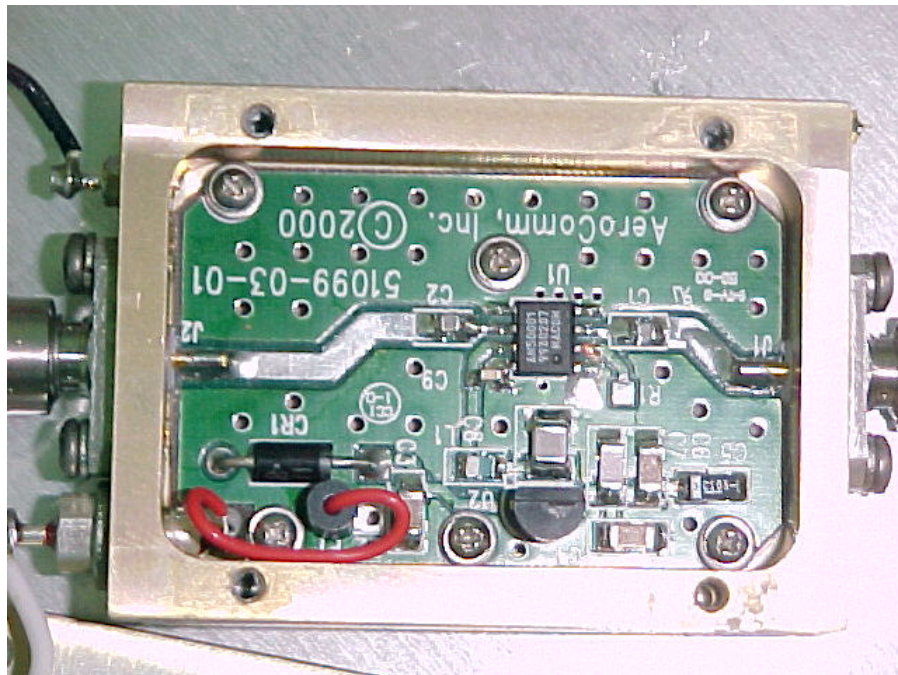
PHOTOGRAPH OF LNA Module Component Side View Model: 51099CELL, S/N 0101-154
