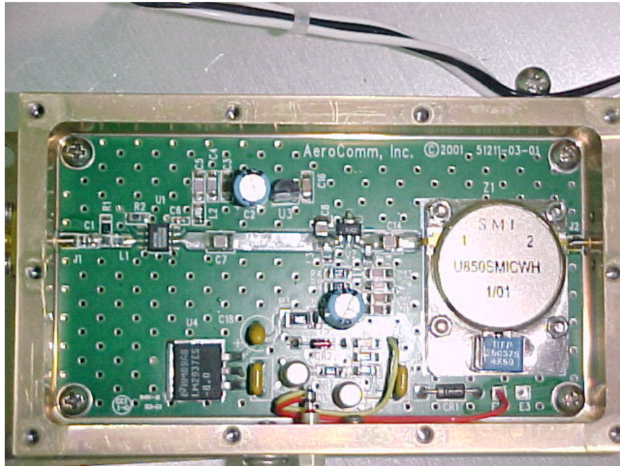
PHOTOGRAPH OF LNA Module Component Side Model: 51211CELL, S/N 0101-79
