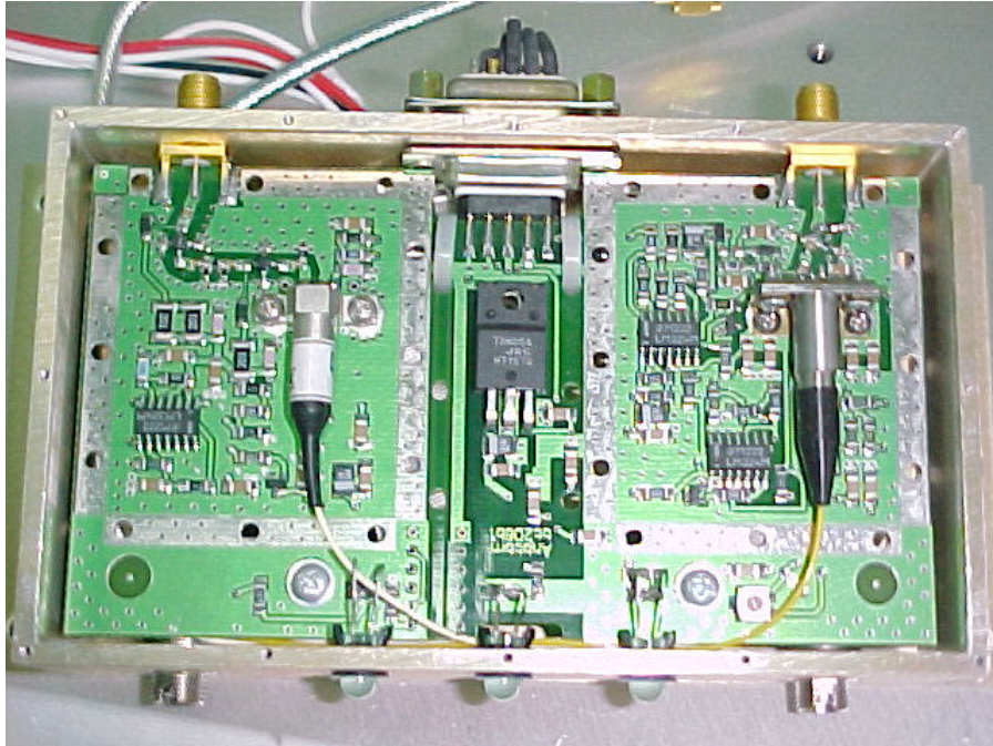
PHOTOGRAPH OF Class 3b Laser Product Soldering Side Model: AC231-A1, S/N 7760122005
