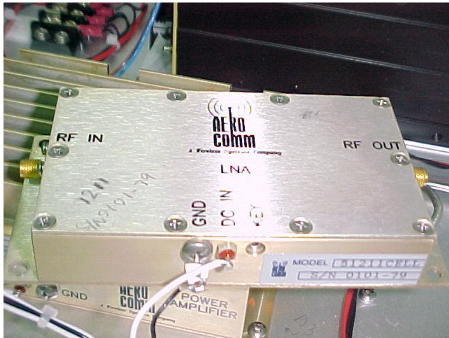
PHOTOGRAPH OF LNA Module Whole View Model: 51211CELL, S/N 0101-79
