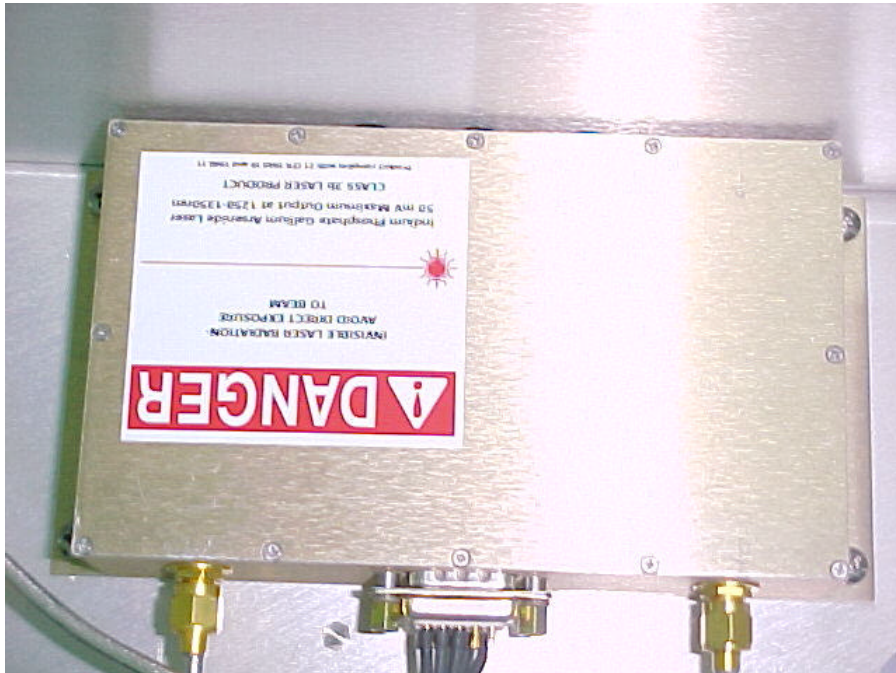
PHOTOGRAPH OF Class 3b Laser Product Whole View Model: AC231-A1, S/N 7760122005
