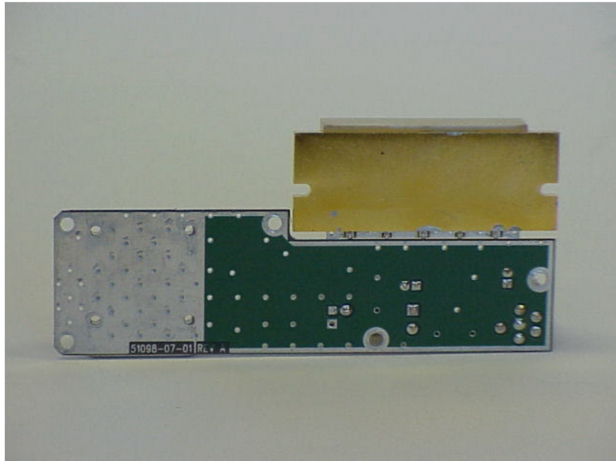
PHOTOGRAPH OF Power Amplifier Component Side View Model: 51098CELL, S/N 0101-190
