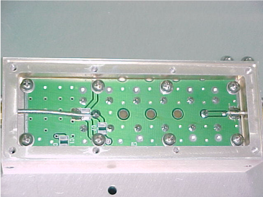
PHOTOGRAPH OF Tx Band Pass Filter Top View 840.5 MHz
