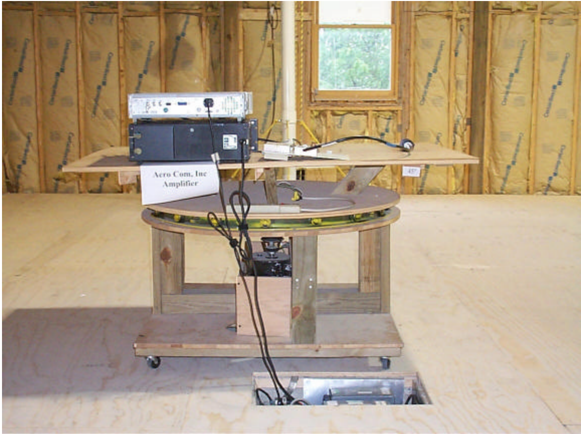
Figure 3:Conducted Emissions
