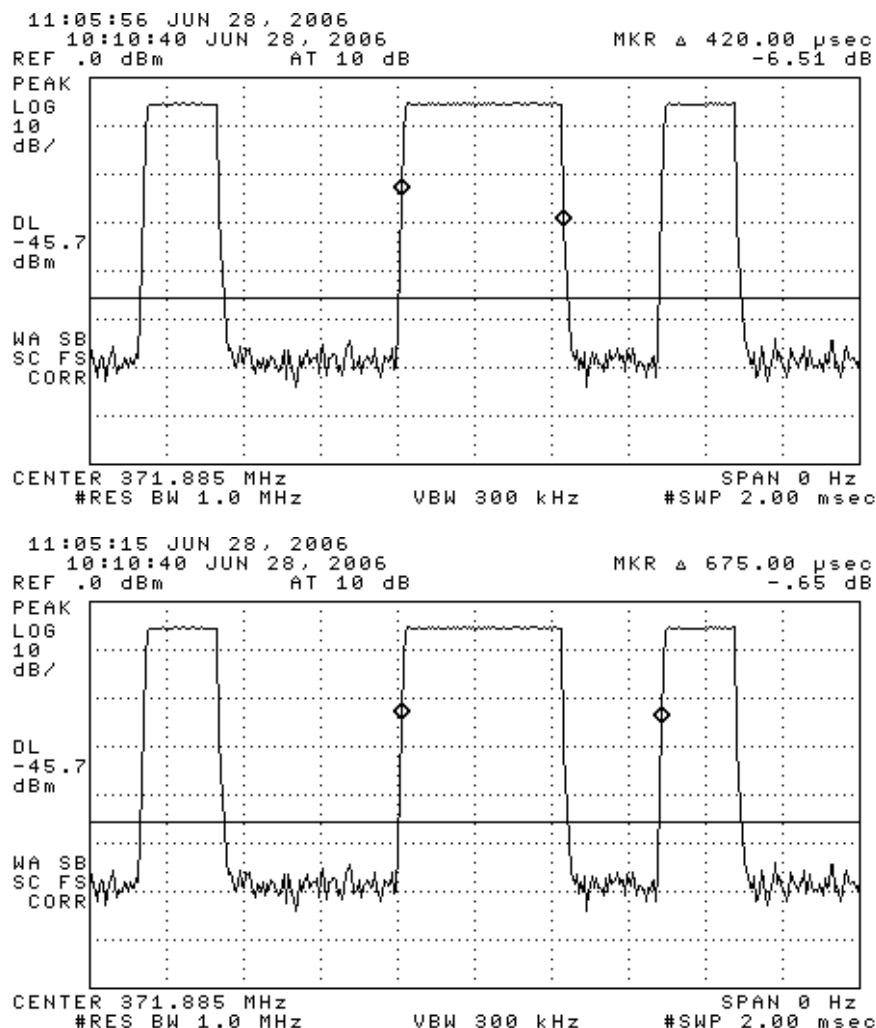
Figure 6.1(a). Transmissions modulation characteristics (cont.).
