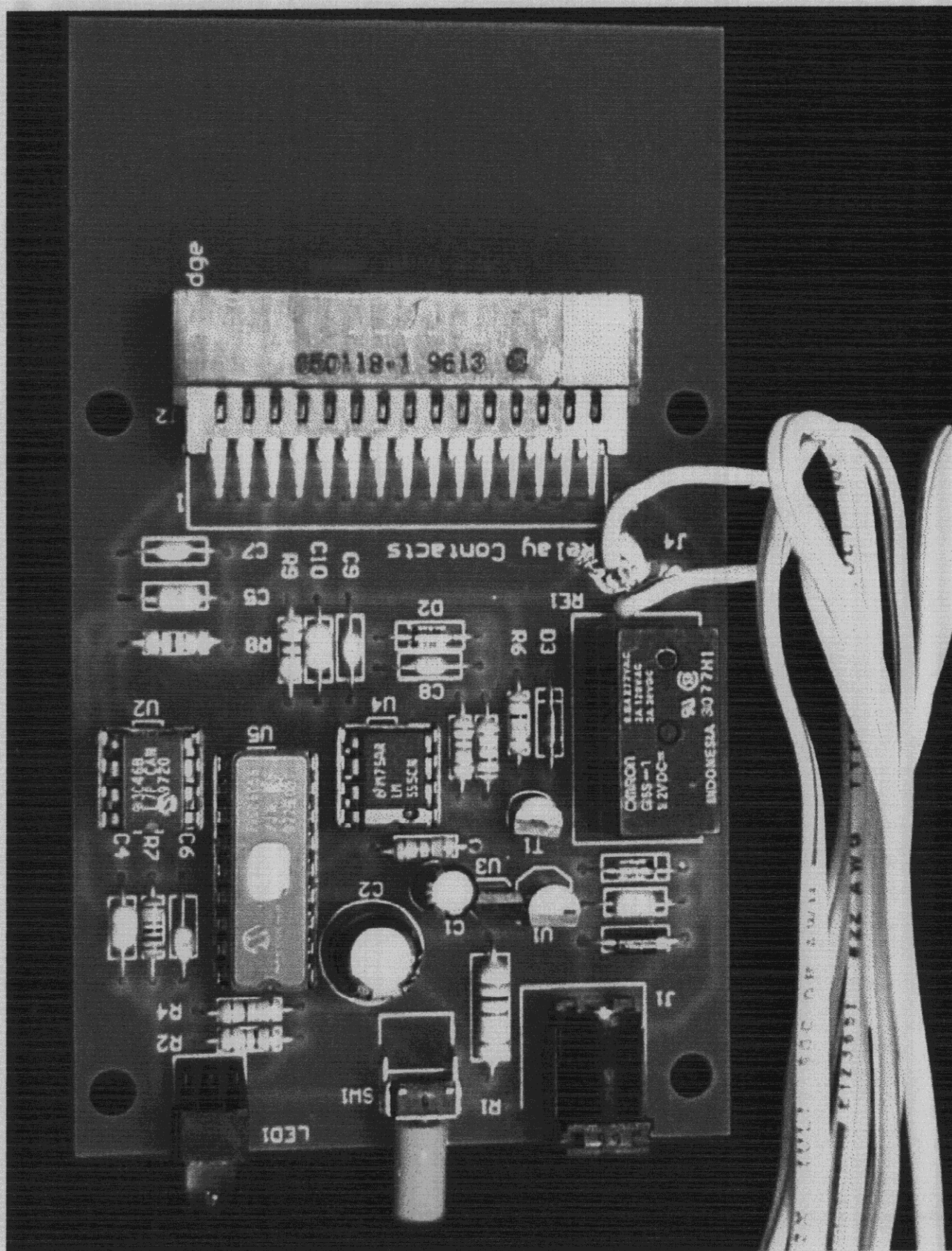
Photo 3. Control Board, Component Side
