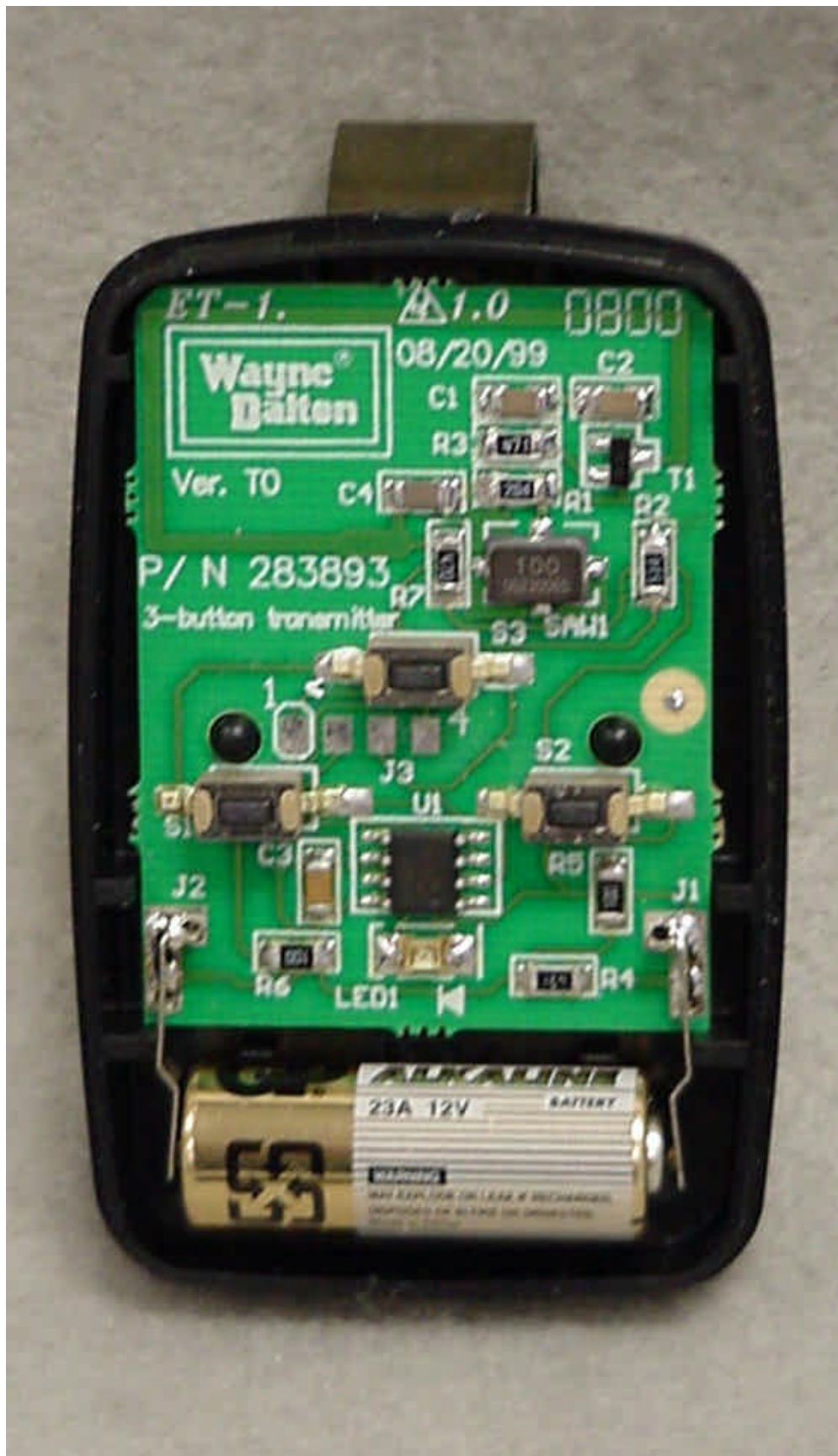
Photo 4. Internal View, Top Side
