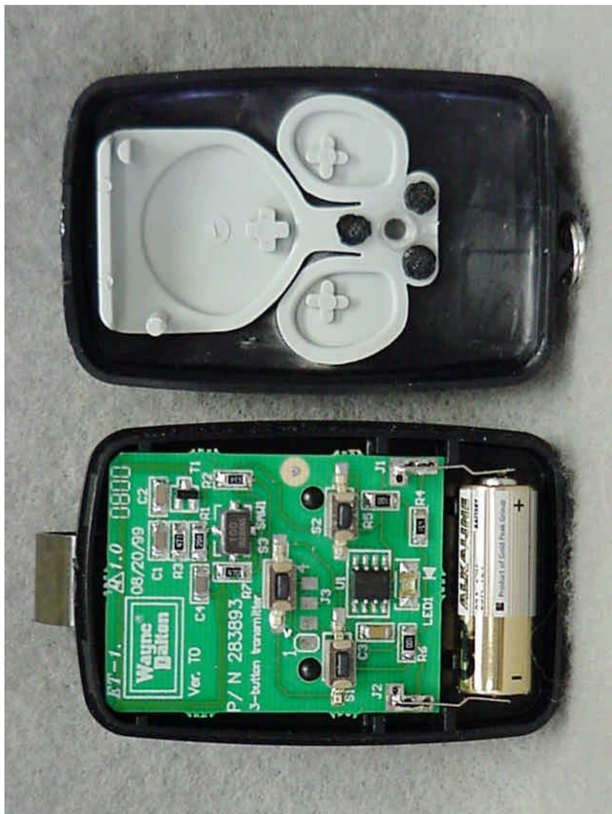
Photo 3. EUT, Cover Opened
