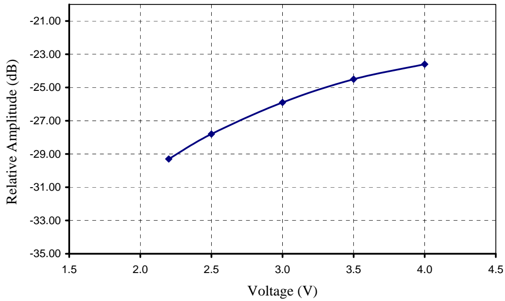
Figure 6.5. Relative emission at 372.0 MHz vs. supply voltage (pulsed emission).
