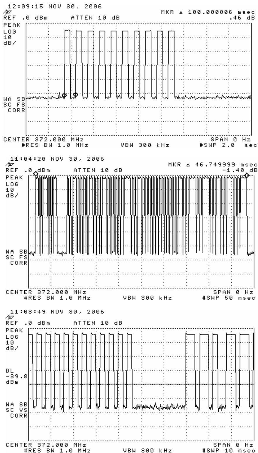
Figure 6.1(a). Transmissions modulation characteristics: (top) complete transmission, (center) expanded dataset, (bottom) expanded wake.
