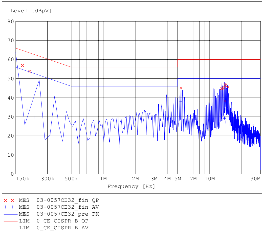
Figure 6.2.1-1: Conducted Emissions Graph – Neutral Line
