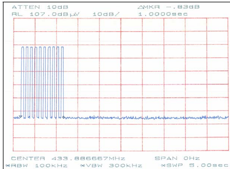
Figure 6.4.3.2-2: Burst Period
