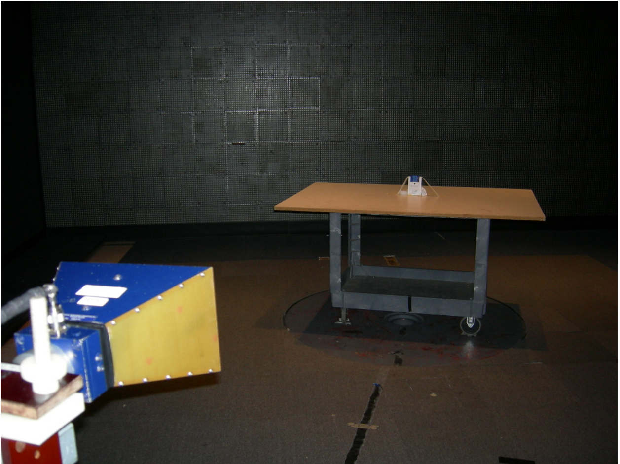
Figure 4: Unintentional Radiated emissions
